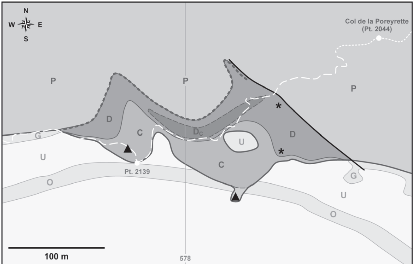
Fig. 2. Map of the paleodoline of La Corde, drawn after aerial photography. Light grey colours: Cretaceous substratum of the structure; Lower Orbitolina Member (O), Upper Schrattekalk Member (U), Garschella Formation (G). Heavy grey line: eocene erosive unconformity, triangles: siderolithic remnants. The sediments of the Sanetsch formation that are filling the paleodoline are given in darker colours: basal conglomerate (C), Diablerets Member (D), “Cerithium Beds” of the Diablerets Member (D c ). The asterisks mark the oyster (north) and coral (south) reefs. The Tsanfleuron Member forming the lid of the paleodoline is traced by the heavy dotted line. The cover of the structure is formed by the Pierredar Member (P). Note the fault cutting off the structure at its northeastern rim (heavy black line). White lines mark the path from Anzeindaz to the Haute Corde peak.
