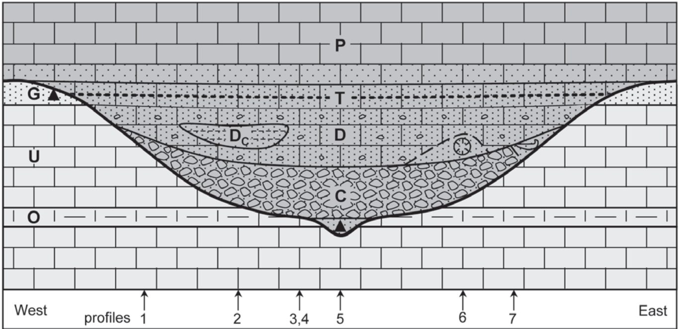
Fig. 6. Simplified, schematic reconstruction of the paleodoline of La Corde in a cross-section, compiled from the profiles 1–7. Abbreviations and symbols as in figures 2 and 5. Note the oyster and coral reefs and the siderolithic relics (triangles) at the bottom and rim of the structure. The sketch is not drawn to scale.
