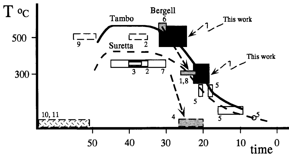
Fig. 4. Temperature-time diagram: the dashed line describes the evolution of the northern and central part of the Suretta nappe and the solid line, the evolution of the central part of the Tambo nappe (Truzzo granite). The dashed arrows describe the temperature-time evolution of the Bergell unit further in the south. See text for explanations. The numbers near the boxes correspond to the data from different authors: (1) K-Ar and Rb-Sr biotite ages, Jäger et al. 1967; (2) K-Ar and Rb-Sr phengite ages, Purdy & Jäger 1976, Steinitz & Jäger 1981; (3) K-Ar phengite ages, Baltzer 1989; (4) Bergell boulders, Giger & Hurford 1989; (5) Zircon and apatite fission tracks, Hurford et al. 1989; (6) U-Pb monazite and zircons, von Blanckenburg 1990; (7) K-Ar phengite ages, Schreurs 1993; (8) K-Ar and Rb-Sr biotite ages, Giger 1991; (9) K-Ar amphibole ages, Flisch & Samsuk in Hurford et al. 1989; (10) Arblatsch flysch deposits, Ziegler 1956 and (11) Eiermann 1988.
