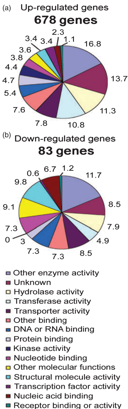
Figure 3. Molecular functions of 761 BABA-responsive genes.
