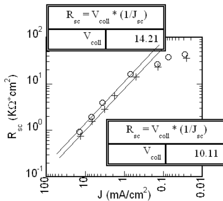
Fig. 5 VIM analysis for the cell of Table 3 (dilution series, X_c \approx 50\% ), before \bullet and after + light-soaking (see Fig. 3 for explanations about VIM analysis)
