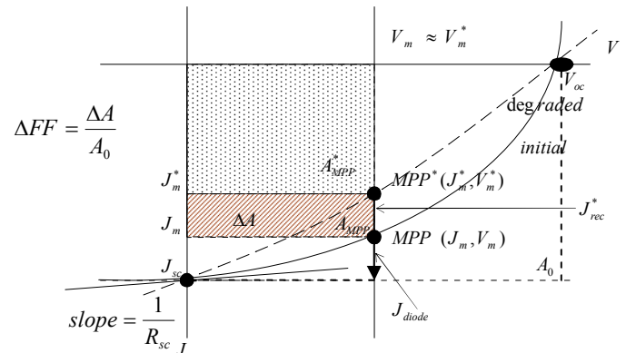
Fig. 2 Schematic representation of J(V) curves for ideal cell and cell with strong recombination losses J_{\text{rec}} .
