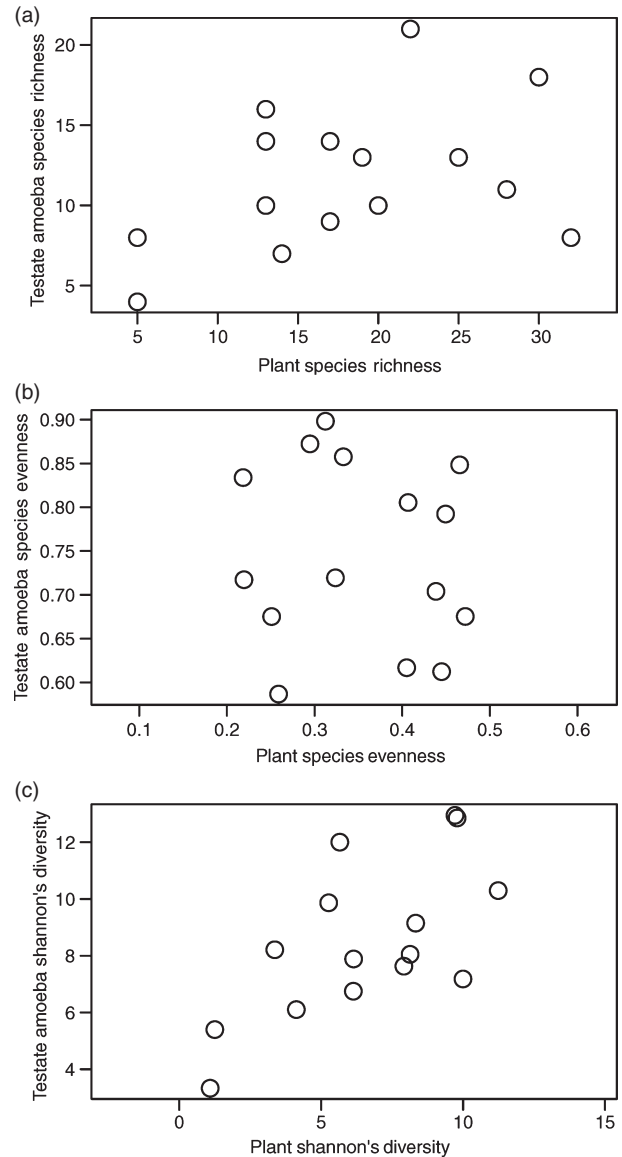
Fig. 3. Relationship between vascular plant and testate amoeba species richness (a), species evenness (b) and Shannon's diversity (c) in the McCarty Fjord chronosequence, Kenai Fjords, Alaska, USA.
