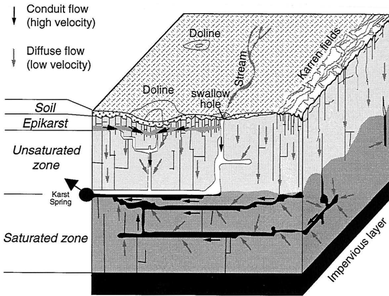
Fig. 1 Conceptual model – scheme – of a karst aquifer used to characterise the vulnerability mapping (Doerfliger and Zwahlen 1995)
