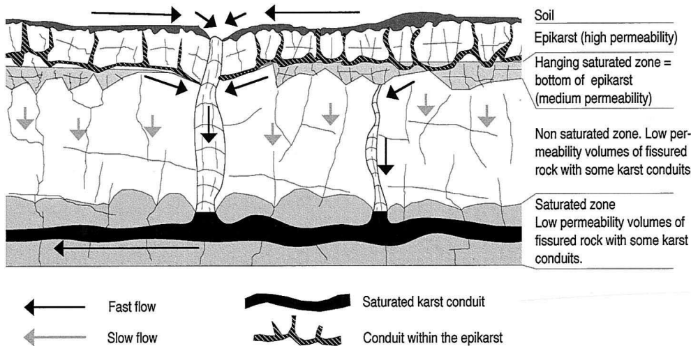
Fig. 2 Water recharge of “low permeability volumes” and of karst conduits by epikarst zone (from Jeannin and Grasso 1995 after Smart and Friedrich 1986)
