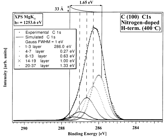
Fig. 8. Experimental and simulated C 1s core levels of the 400°C annealed, high nitrogen-doped diamond (100) surface. Agreement is achieved for a band bending value of 1.65 eV. The peaks formed by markers are the sum of the peaks formed by every layer from the surface to the bulk (listed in the legend). The corresponding C 1s band is shown above the graph.
