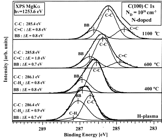
Fig. 7. XP normal emission spectra ( \text{MgK}\alpha , h\nu = 1253.6 \text{ eV} ) of the C 1s core level obtained after heating the high nitrogen-doped diamond with hydrogen-terminated (100) surface to temperatures up to 1100^\circ\text{C} .
