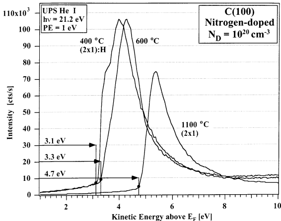
Fig. 13. Low kinetic-energy part of the He I ( h\nu = 21.2 eV) normal emission spectra after heating the H-terminated high nitrogen-doped diamond (100) surface to temperatures up to 1100 °C. The energy scale is corrected for an applied bias voltage of -1.5 V to overcome the work function of the analyzer.
