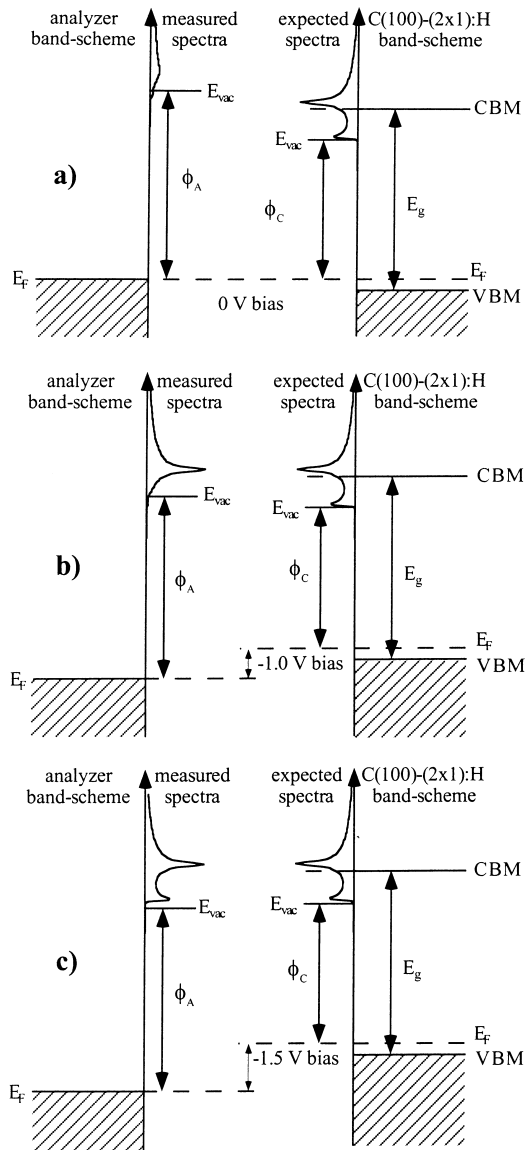
Fig. 5. Emission model showing on the right side the He I ( h\nu = 21.2 eV) normal emission spectrum of the valence band for the diamond (100)-(2 \times 1):H surface with the corresponding energy band diagram, and on the left side, the evolution of the measured spectra with increasing applied voltage [from 0 to -1.5 V corresponding to (a)– (c)].
