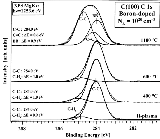
Fig. 6. XP normal emission spectra ( \text{MgK}\alpha , h\nu = 1253.6 \text{ eV} ) of the C 1s core level obtained after heating the high boron-doped diamond with hydrogen-terminated (100) surface to temperatures up to 1100^\circ\text{C} .
