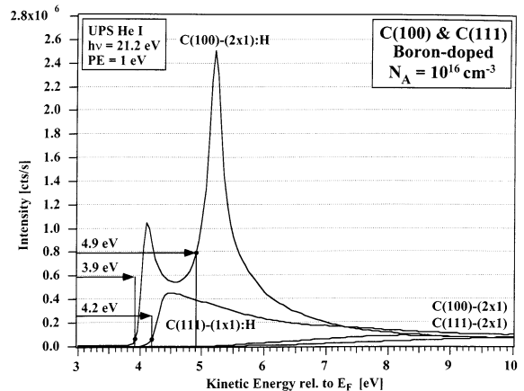
Fig. 9. Low kinetic-energy part of the He I ( h\nu=21.2 eV) normal emission spectra showing the valence band of the H-terminated and H-free low boron-doped diamond (100) and (111) surfaces. The energy scale is corrected for an applied bias voltage of -1.5 V to overcome the work function of the analyzer.
