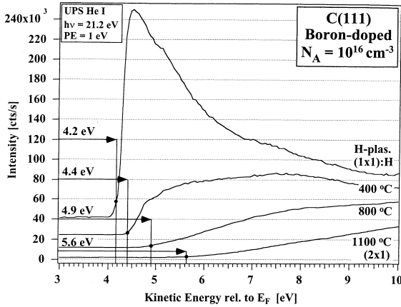
Fig. 11. Low kinetic-energy part of the He I ( h\nu=21.2 eV) normal emission spectra after heating the H-terminated low boron-doped diamond (111) surface to temperatures up to 1100°C. The energy scale is corrected for an applied bias voltage of -1.5 V to overcome the work function of the analyzer.
