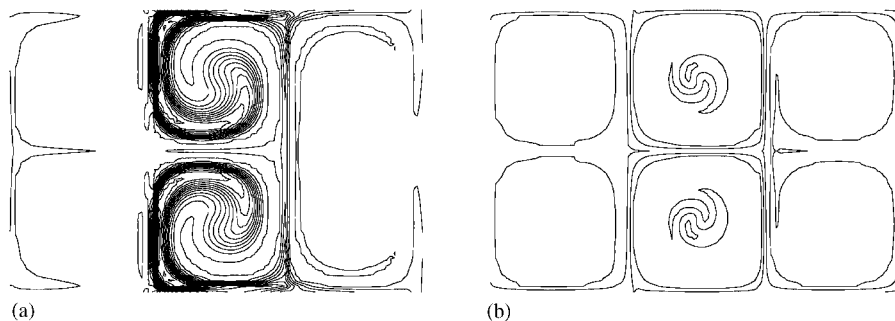
Figure 11. (a) Streamline diffusion and shock capturing (200th step). (b) Streamline diffusion and shock capturing (800th step).
