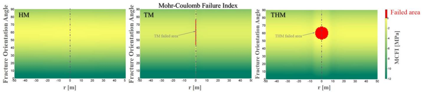
Fig 7. Profiles of the Mohr-Coulomb fracture index for 0-90 degrees range of the fracture orientation under three different injection scenarios, i.e. HM, TM and THM cases after 20 hours. The red color represents positive MCFI , indicating failure has occurred.
