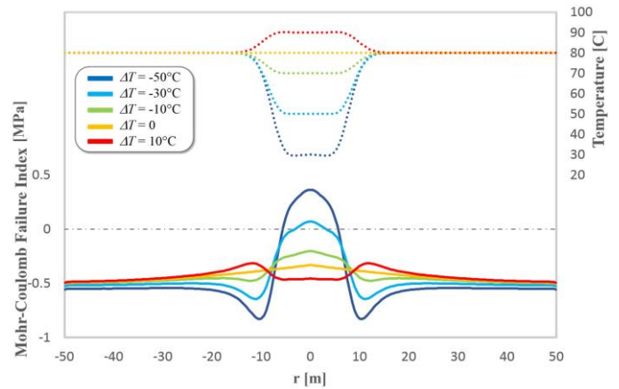
Fig 10. Profiles of Mohr-Coulomb failure index (solid lines) and temperature (dotted lines) along the fracture at the end of injection/cooling (i.e. 20 hours) for different injection temperature. The gray dash-dotted horizontal line at MCFI = 0 denotes the M-C failure line.
