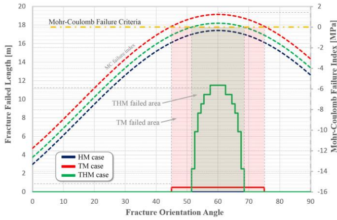
Fig 8. Fracture failed length (solid lines) and Mohr-Coulomb failure index (dashed lines) as a function of fracture orientation. The green and red shaded areas denote the range of failure orientations for the THM and TM cases. The yellow dash-dotted horizontal line at MCFI = 0 denotes the M-C failure line.
