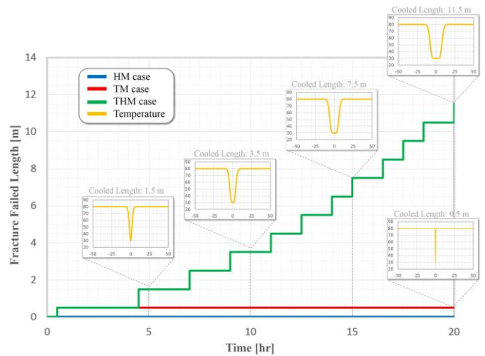
Fig 5. Evolution of the failed length of the fracture (includes both sides) based on the M-C criterion over 20 hours of fluid injection and/or cooling for the three cases. The profiles of temperature along the fracture for several times are shown by the insets. A reasonable correlation between cooled length and fracture failed length is achieved.
