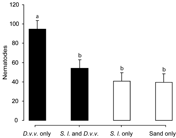
Figure 5 Mean ( \pm SE) number of nematodes recovered from the six treatment arms of the belowground olfactometer; containing a plant attacked by 4 D. v. virgifera larvae ( D. v. v. only), a plant attacked by 20 S. littoralis and 4 D. v. virgifera ( S. l. and D. v. v. ), a plant attacked by 20 S. littoralis ( S. l. only), and humidified sand only (Sand only). The ‘Sand only’ bar is obtained by averaging the mean number of nematodes choosing the three arms containing only sand. Different letters above bars indicate differences in the choices made by the nematodes for the different treatments ( n = 12 , P < 0.05 ).
