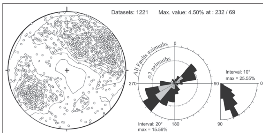
Fig. 8. Stereographic representation of all the fault measurements used in this study, with the corresponding density diagrams (equal area of the poles of the plane projections, lower hemisphere). The maximum density value is obtained at (az=232; pl=69).
