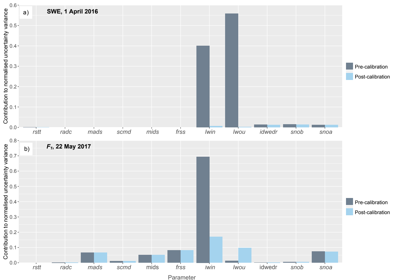
Fig. 8. Parameter contributions to predictive uncertainty variance pre- and post-calibration for the predictions of a) Snow Water Equivalent on 1 April 2016, and b) snow pattern (summarised by F_1 ) on 22 May 2017.
