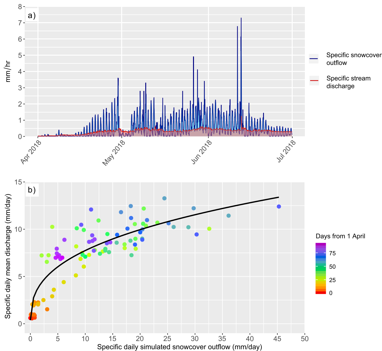
Fig. 7. a) Simulated hourly specific (i.e. catchment-averaged) “snowcover outflow” (i.e. snowmelt from non glaciated areas, plus any liquid precipitation) vs. hourly observed stream specific discharge for the Vallon de Nant sub-catchment during spring 2018 (discharge gauged at Avancon Weir and normalised according to catchment area), and (b) simulated daily sum specific “snowcover outflow” vs. observed daily mean specific stream discharge, again at the Avancon Weir station, over the same 3-month period.
