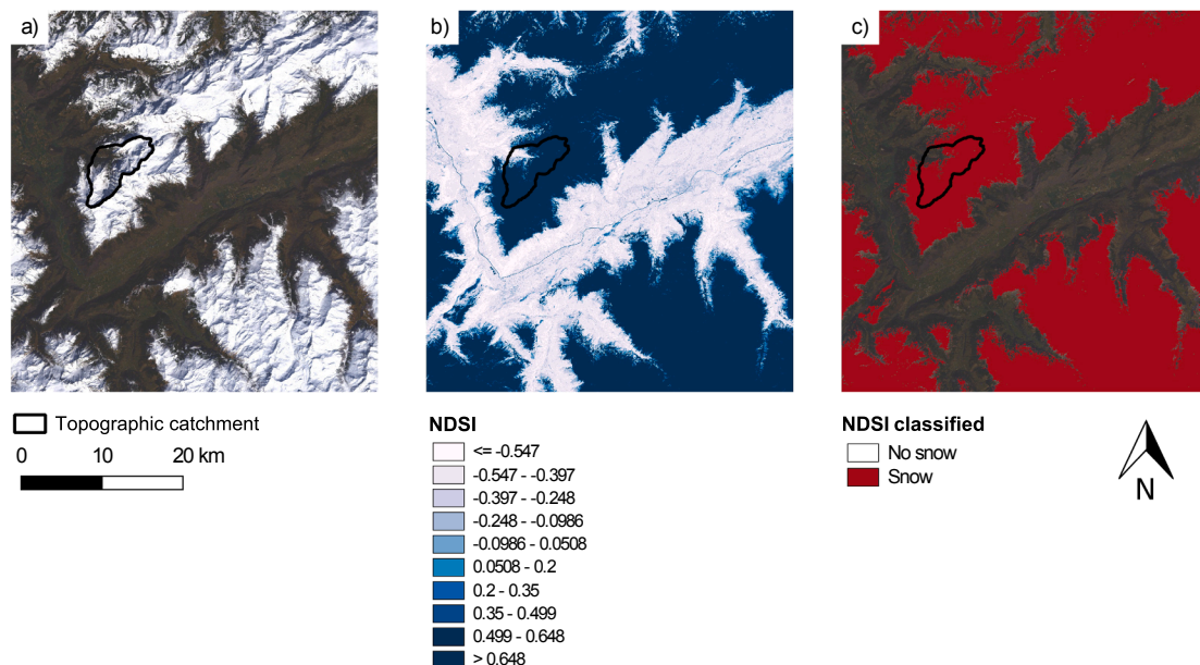
Fig. 2. Illustration of the binary snow extent map generation process, taking the 8 April 2015 as an example: a) True Colour Composite, b) calculated NDSI raster, and c) final binary observed extent developed by identifying and applying a threshold to (b). Each image in the catalogue was inspected and classified individually.
