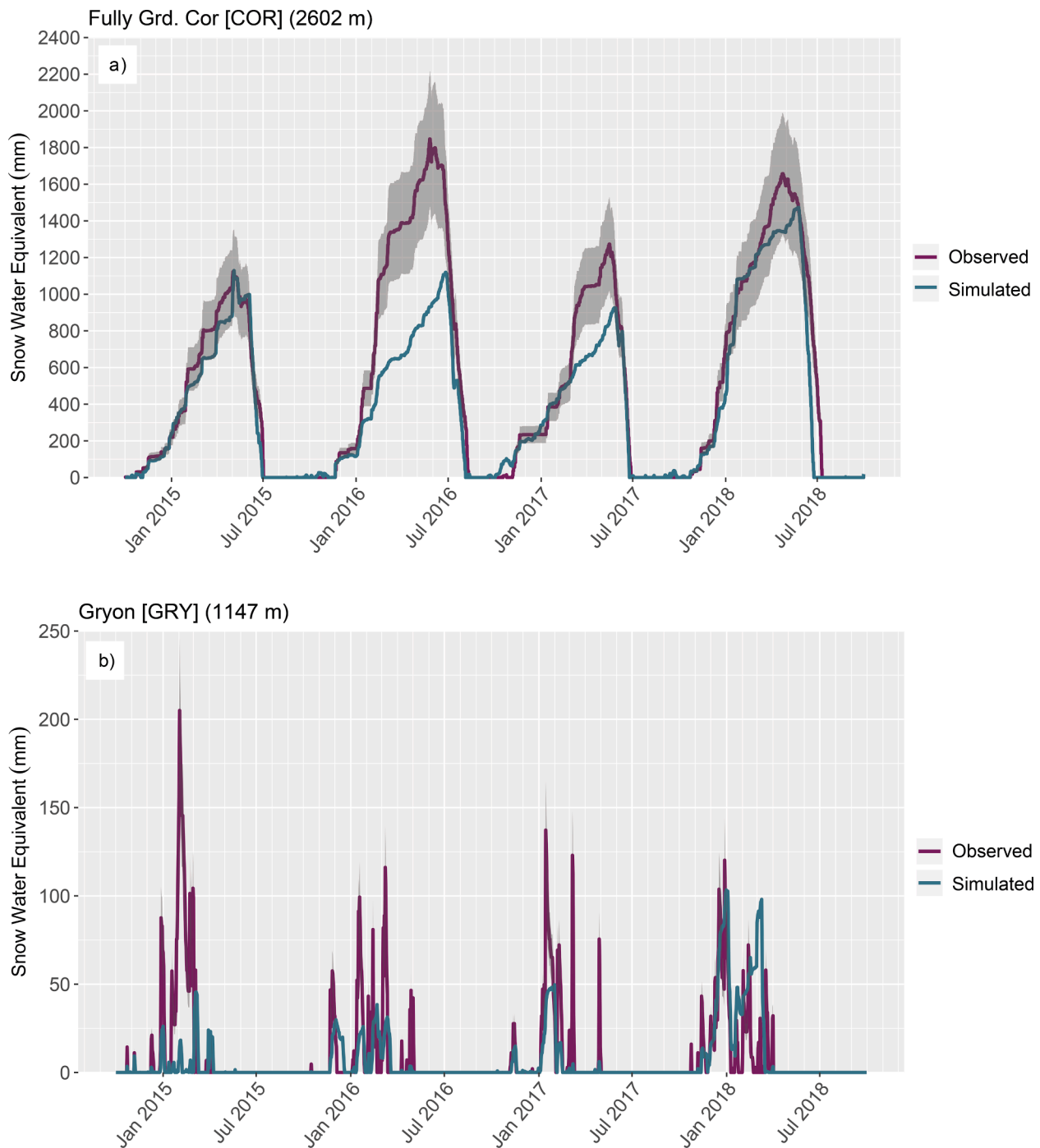
Fig. 4. Observed and simulated Snow Water Equivalent (SWE) time-series at the two measurement stations, Fully Grand Cor (a: COR, hourly) and Gryon (b: GRY, daily). The observations are not direct measurements of SWE, but rather are reconstructions based on snow depth and other measurements at COR, and purely snow depth at GRY. The grey bar of \pm 20\% is added around the reconstructed “observed” series to reflect the pixel-point nature of these comparisons.
