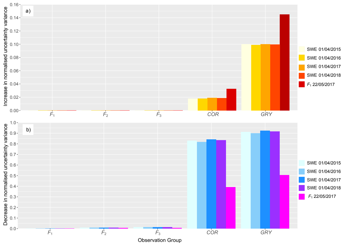
Fig. 9. a) Increase in relative (to the pre-calibration uncertainty variance) post-calibration predictive uncertainty variance associated with each of the five selected predictions incurred by omitting each observation group from the calibration dataset in turn, and b) decrease in relative (again to the pre-calibration uncertainty variance) uncertainty variance accrued when each observation group comprises the sole member of the calibration dataset. The “redundancy”, or commonality of information, between the three spatial observation groups (i.e. F_1 , F_2 , and F_3 ) is clearly apparent.
