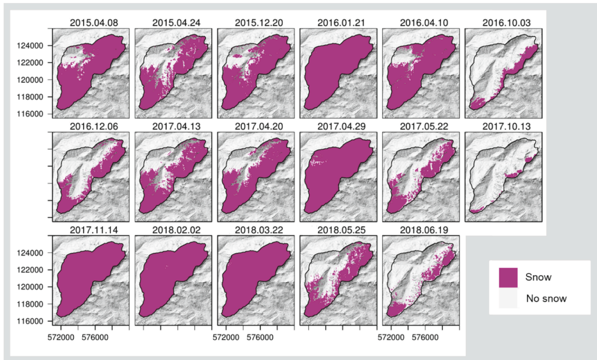
Fig. 3. The complete catalogue of 30-metre resolution observed snow extent maps compiled. The date of each image is indicated. Coordinates are in the CH1903 system.
