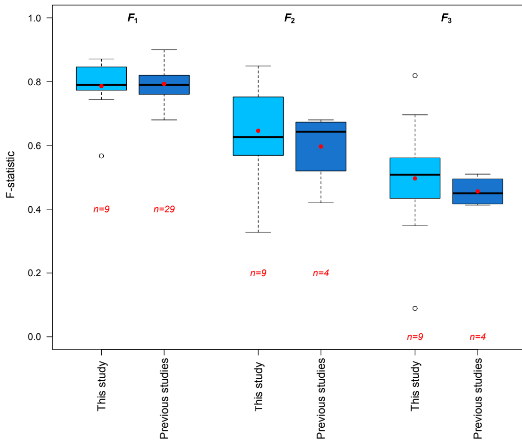
Fig. 5. Comparison between the spatial model fits obtained in the present study and previously reported equivalents (i.e. the same metrics generated with respect to Landsat imagery). In the interests of fairness, only the F-statistics from this study that corresponded to spring and early summer (i.e. 08/04/2015, 24/04/2015, 10/04/2016, 13/04/2017, 20/04/2017, 29/04/2017, 22/05/2017, 25/05/2018, 19/06/2018) are included. The medians are represented using a thick black line in the traditional fashion, whilst the red dots indicate the means. (For interpretation of the references to colour in this figure legend, the reader is referred to the web version of this article.)
