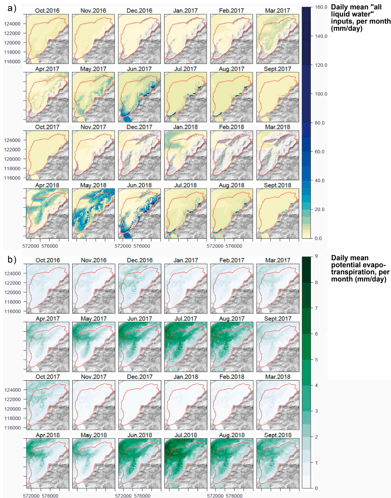
Fig. 6. Simulated spatio-temporal patterns of a) "all liquid water" arriving at the surface (i.e. liquid precipitation + snowmelt + firn melt + ice melt), and b) potential evapotranspiration ( ET_p ) generated using the optimised model configuration over the two hydrological years 2017–2018. The underlying hourly data are expressed here as daily mean values in mm, averaged across calendar months.
