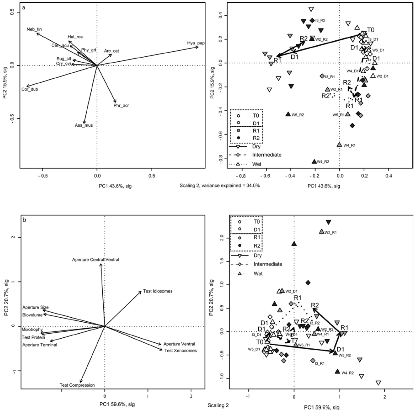
Fig. 2. Principal component analyses (PCA) of a ) testate amoeba species and b ) community weighted mean (CWM) of functional traits in Sphagnum fallax from a mesocosm experiment simulating water table changes. The species dataset was Hellinger transformed and the CWM data were scaled. Projection of descriptors (left) and samples (right), scaling 2. On the right plots, arrows represent the time line for each treatment (mean coordinates of the five sampling plots of each treatment and time). In both PCAs, axes 1 and 2 were the only significant axes and accounted respectively for 60.4% (species based) and 80.2% (CWM based) of the variance. Characteristic plots for wet and intermediate treatments were labelled. Taxa abbreviations: Amp_wri: Amphitrema wrightianum , Pse_gra: Pseudodiffugia gracilis , Arc fla: Archerella flavum , Cyc_arc: Cyclopyxis arcelloides , Phy_gri: Physochila griseola , Hya_pap: Hyalosphenia papilio , Cen_acu: Centropyxis aculeata , Hel_syl: Heleopera sylvatica , Cry_ovi: Cryptodiffugia oviformis , Eug_cil: Euglypha ciliata , Phr_acr: Phryganella acropodia , Hel_ros: Heleopera rosea , Cor_dub: Corythion dubium , Neb_tin: Nebela tincta s.l., Arc_cat: Arcella catinus , Ass_mus: Assulina muscorum .
