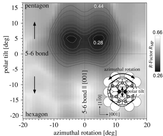
FIG. 3. R -factor plot obtained by azimuthal rotation and polar tilt of the C_{60} molecules away from the symmetric 5-6 orientation. Inset: Schematic drawing defining the angles used to describe the rotations. For clarity, only the carbon atoms closest to the surface are shown.
