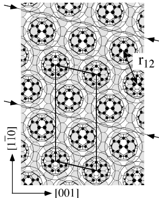
FIG. 2. Structural model for the C_{60} monolayer on Cu(110). For clarity, only the carbon atoms closest to the surface are shown as solid dots, with a size proportional to their proximity to the substrate surface. In order to indicate the distortion from a perfect hexagonal layer, circles whose radii corresponds to half the C_{60} - C_{60} NN spacing in bulk C_{60} ( 5.02 Å) are drawn around the molecules. Only one of the two possible domain orientations (unit cell indicated) and inequivalent azimuthal orientations of the molecules ( \pm 180^\circ ) are shown. Arrows indicate the larger separation between adjacent rows occurring every three rows. The short r_{12}=9.6 Å intermolecular distance is indicated.
