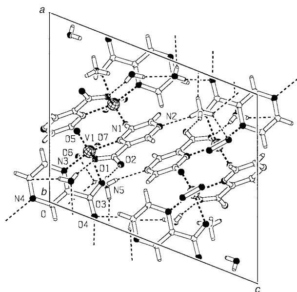
Fig. 5 Representation of the unit cell of [\text{NH}_4]\text{[VO(O}_2)(\text{pca})_2] .
