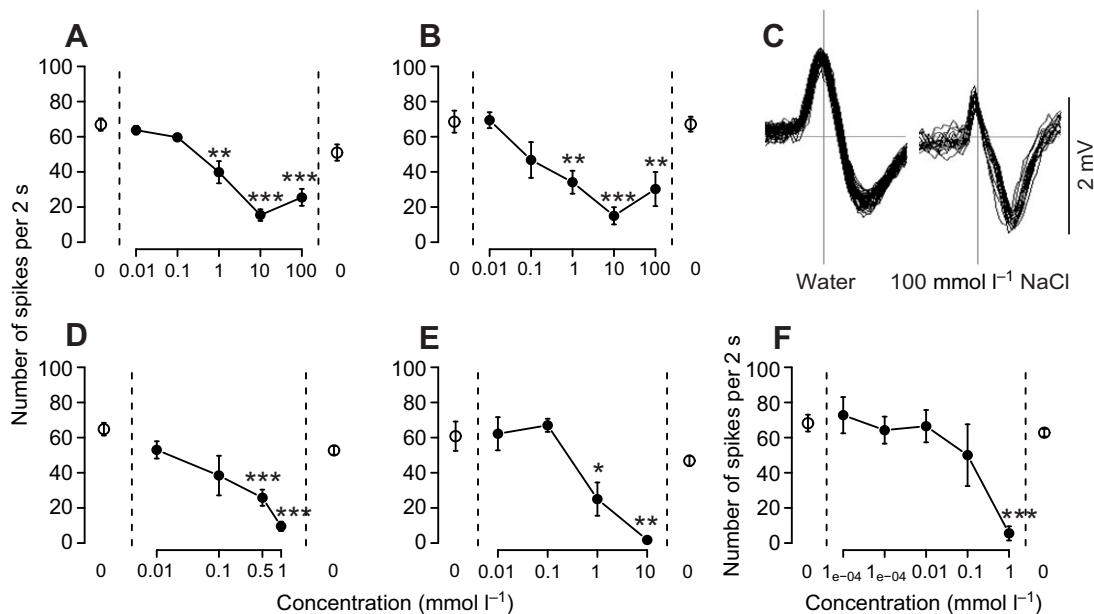
Fig. 7. Mean \pm s.e.m. total number of spikes generated by sensory cells within trichoid T1 sensilla on the labellum of female A. gambiae during stimulation by water as a function of the log 10 concentrations of (A) KCl (12 mosquitoes tested), (B) NaCl (10 mosquitoes tested), (D) CuSO 4 (five mosquitoes tested), (E) CaCl 2 (five mosquitoes tested) and (F) LaCl 3 (four mosquitoes tested). (C) Superimposition of action potentials recorded during stimulation with water (left) and with 100 mmol l -1 NaCl (right) displaying differences in shapes and amplitudes of the generated action potentials. Asterisks indicate numbers of spikes generated by the water neurone that are significantly lower than for the initial water controls (presented on the left of each graph); Welch's t -test, * P <0.05, ** P <0.01, *** P <0.001.
