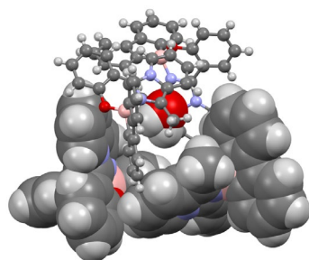
Figure 2. Cubic structure formed by four molecules of 3a (two ball and stick and two space filling representations) showing a water molecule (space filling) sitting inside the cavity. Color code: dark grey: carbon atoms, light grey: hydrogen atoms, red: oxygen atoms, light blue: nitrogen atoms, pink: boron atoms.
