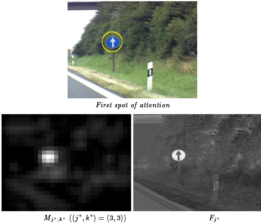
Fig. 4. The segmentation-relevant data provided by MAPS about the first spot of attention on a traffic scene image. M_{3,3} is the multiscale conspicuity map with the highest conspicuity value around this spot. Thus, F_3 (opponent colors B/Y ) is the most discriminating feature of this location.
