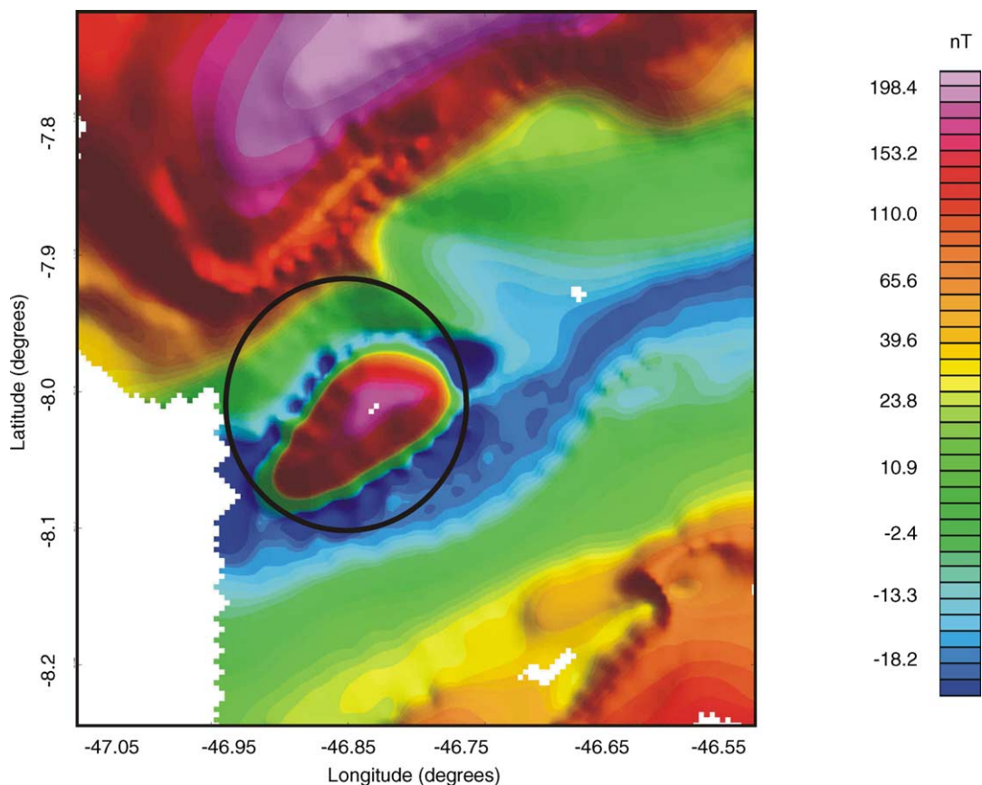
Fig. 13. Reduced to pole residual aeromagnetic map of the Serra da Cangalha impact crater region downward continued to 1.1 km. The circular structure at the centre represents the impact crater region. In comparison with Figs. 15, the uplifted basement is clearly evident from this map.
