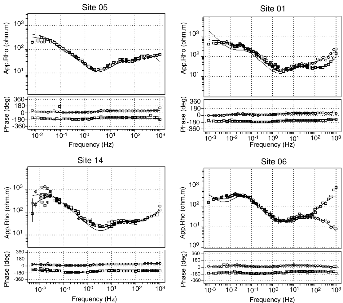
Fig. 4. Examples of apparent resistivity and phase curves calculated from the impedance tensor after rotation to the direction of the regional strike. The panels on the left are MT sites located away from the crater center. The right panels are MT sites located close to the crater center.
