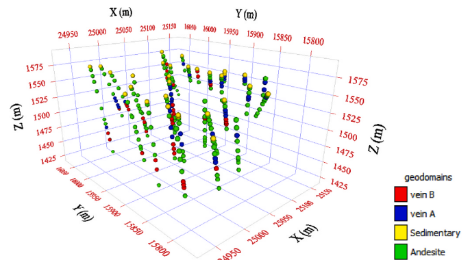
Fig. 1. Isoclinal view of the conditioning borehole dataset. The spheres represent centroids of the intervals logged for lithology.
