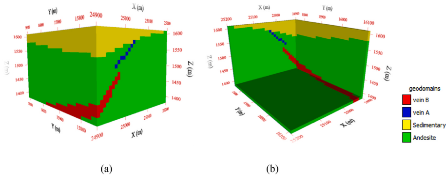
Fig. 3. Block model of the gold deposit: (a) 3D view, (b) cross-sectional view.
