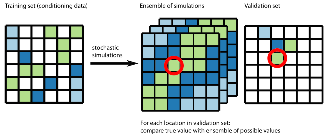
Figure 3. Example of one cross-validation iteration. The domain is simulated n_r times with conditioning data (ensemble of simulations is obtained). Each point in the validation set is compared with vector p constructed by aggregating realizations in the ensemble.
