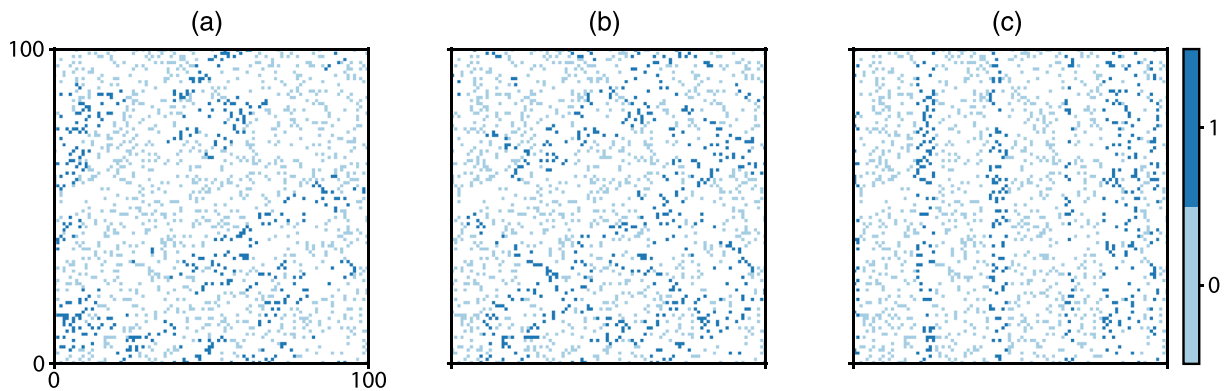
Figure 6. Example of synthetic observation sets obtained by sampling from each of the synthetic realities (a, b, c). Here each synthetic observation set contains 1,600 samples.
