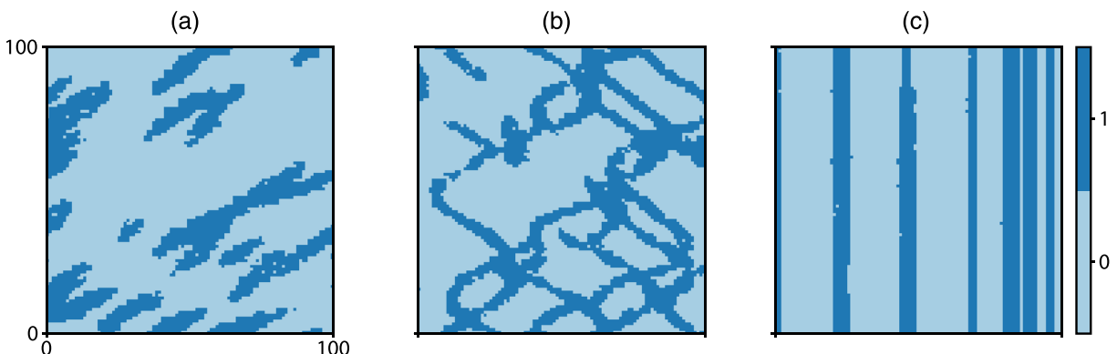
Figure 5. Three synthetic realities, each obtained by means of DeeSse simulation using training images (a, b, c).
