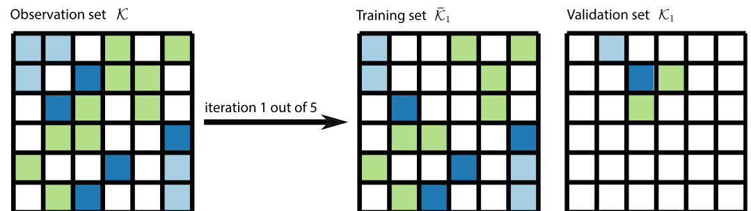
Figure 2. The split of the example data ( \mathcal{K} ) in a regular grid in the first cross-validation iteration. The first subset ( \mathcal{K}_1 ) becomes the validation set, and the complementary data set (training set, \bar{\mathcal{K}}_1 ) becomes the conditioning data for the geostatistical model.
