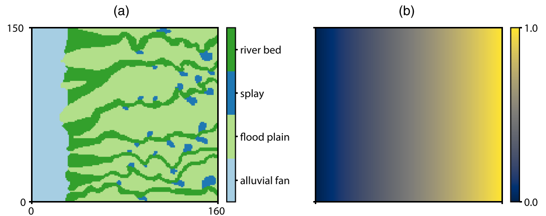
Figure 10. The analog training image (a) with its corresponding trend (b). The training image contains four geological facies.
