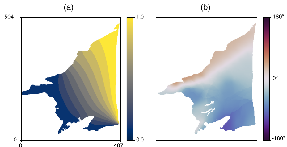
Figure 7. Area of the multivariate simulation with defined trend (a) and orientation (b).
