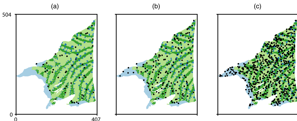
Figure 9. The synthetic reality obtained by DeeSse simulation using the reference TI and samples locations: (a) 50 wells, (b) 150 wells, and (c) 600 wells, representing synthetic observation data sets.
