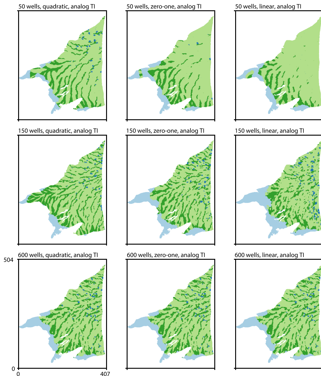
Figure 14. Example simulations with the analog TI, the best DeeSse parameters found with cross-validation for each observation set (50, 150, and 600 wells), and different scoring methods (quadratic score, zero-one score, and balanced linear score).
