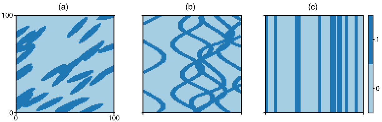
Figure 4. Three training images of type (a) ellipsoids, (b) waves, and (c) stripes used in the benchmark of training image selection (data from Pérez et al., 2014).
