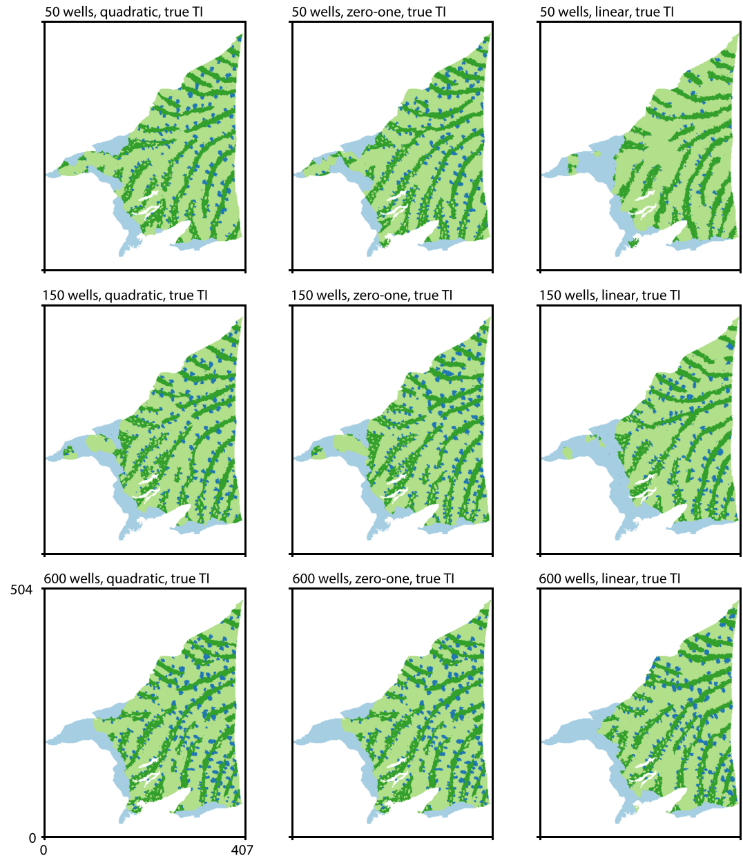
Figure 13. Example simulations with the reference TI, the best DeeSse parameters found with cross-validation for each observation set (50, 150, and 600 wells), and different scoring methods (quadratic score, zero-one score, and balanced linear score).
