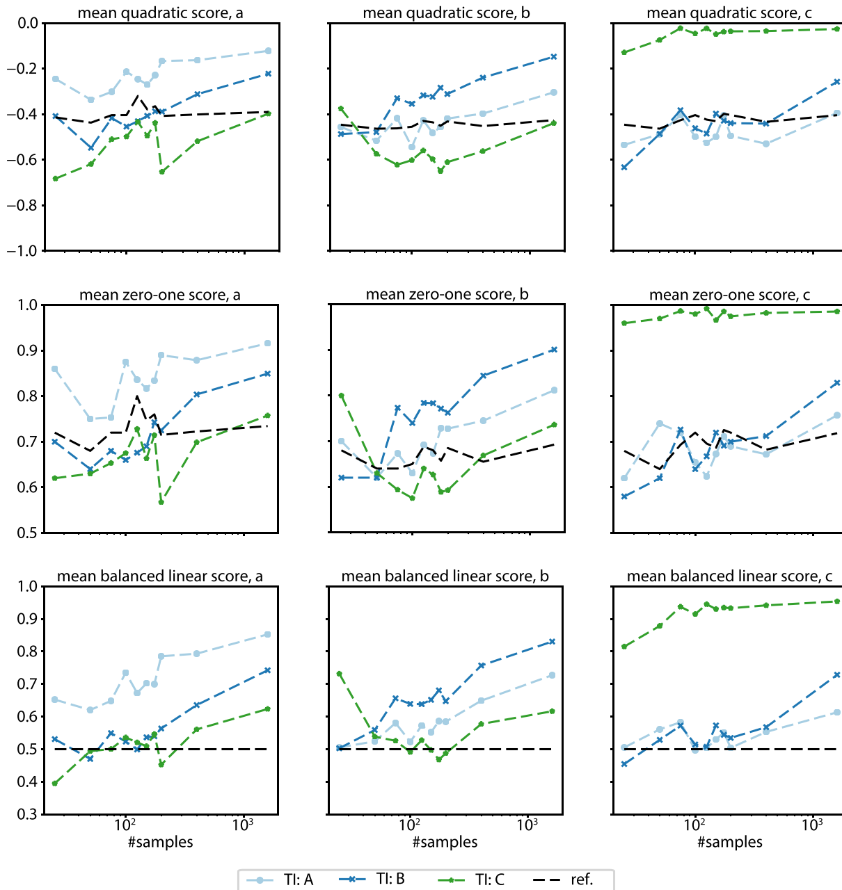
Figure 12. Cross-validation scores for synthetic observations with respect to the number of samples in the data set for each of the different types of observation sets (a, b, c). Thirty realizations per fold were generated. Mean quadratic score, mean zero-one score, and mean balanced linear score were used.
