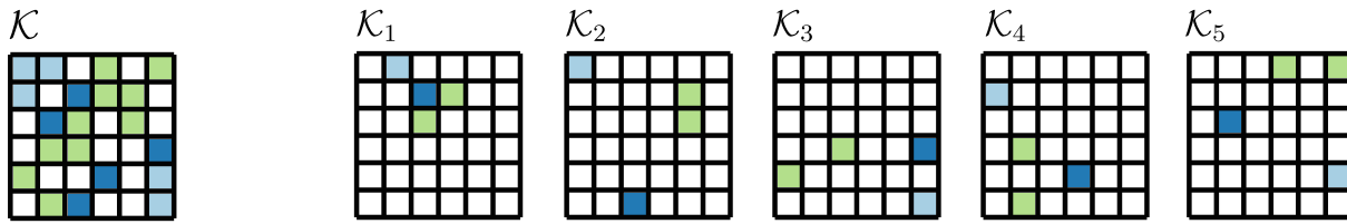
Figure 1. Example of shuffled fivefold stratified split of data ( \mathcal{K} ) in a regular grid belonging to three classes (light blue, dark blue, and green).
