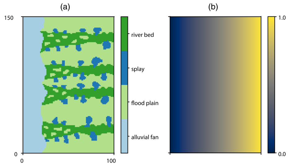
Figure 8. The reference training image (a) with the defined trend (b). The training image contains four geological facies.
