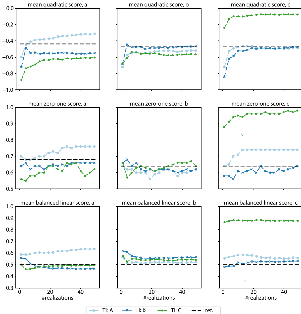
Figure 11. Sensitivity study with respect to the number of realizations per fold for each of the different types of observation sets (a, b, c). Each of the samples contained 50 observations. Mean quadratic score, mean zero-one score, and mean balanced linear score were used.
