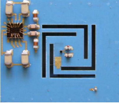
Fig. 11. LTCC substrate with VCSEL island, bonded ASIC, impedance matching network, and transmission line through suspension arm. Overall LTCC substrate size is 14 mm \times 16 mm.
