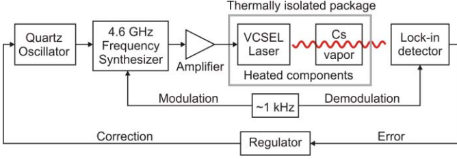
Fig. 1. Atomic interrogation loop of a CPT-based clock.
