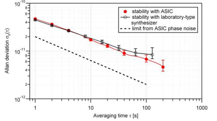
Fig. 13. Clock stabilities recorded with the experimental clock setup, using the reference synthesizer (open symbols) and the ASIC synthesizer (filled symbols). The dashed line is the theoretical limit from ASIC phase noise.
