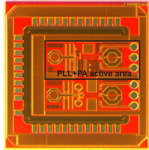
Fig. 4. Die microphotography with a PLL+PA active area of 0.7 mm 2 .
