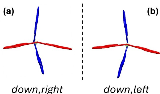
Figure 5. Inherent chirality in [\text{Zn}(\text{L}^{\text{Me}})_2]^{2+} generated by ligand concavity. Red and blue sketches represent the two bis(imidazo[1,5- a ]pyridine)methane ligands; zinc center in light green. The terms down, right and left indicate the concavity of the ligands. Arbitrarily, the concavity of the red ligand is reported first, followed by the concavity of the blue ligand. Thus, the two enantiomers can be described as down, right or down, left .
