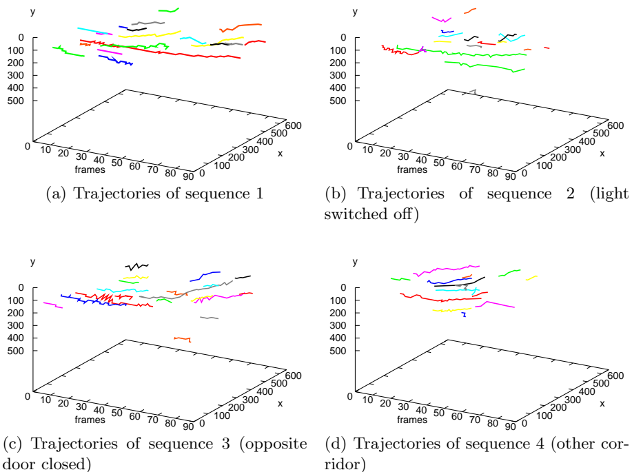
Fig. 6. Trajectories of the tracked spots of attention from four different sequences ((a)..(d)). Note that only trajectories with Card(T) > 3 are represented here.
