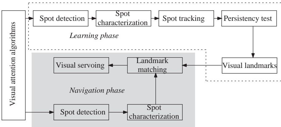
Fig. 1. Overview of the attention-based landmark selection approach.
