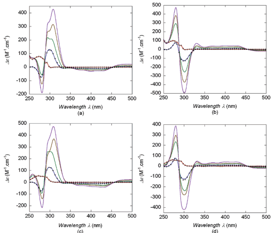
Figure 5. Refined CD spectra for each absorbing species for (\Lambda\text{-}1)_x\text{C} streptavidin (a), (\Delta\text{-}1)_x\text{C} streptavidin (b), (\Lambda\text{-}1)_x\text{C} avidin (c), and (\Delta\text{-}1)_x\text{C} avidin (d). Key: x = 0 , red line; x = 2 , green line; x = 3 , brown line; x = 4 , violet line. For comparison, the measured spectra for the host protein and for the biotinylated guest 1 are displayed as open circles and full triangles, respectively, overlaid with the corresponding refined spectra (thin lines).
