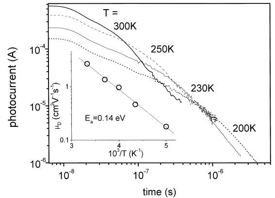
Fig. 2. Temperature dependence of the electron time-of-flight transients at U_{\text{appl}} = 2 \text{ V} . The inset illustrates the thermally activated behaviour of the electron mobility together with a fit corresponding to activation energy E_a = 0.14 \text{ eV} .
