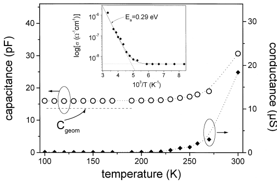
Fig. 4. Temperature dependence of the capacitance (open circles, left axis) and conductance (full diamonds, right axis) of the 5.6 \mu\text{m} \mu\text{c-Si:H} sample measured at f = 100 \text{ kHz} . Experimental points are connected by dotted lines as a guide to eye. At low temperatures the capacitance approaches the geometrical value (dashed line calculated for \epsilon_{\text{Si}} = 11 ). The increase of capacitance with T seems to be related to the simultaneous increase of the thermally activated conductance (see inset with the conductance data replotted in log scale together with a fit by a sum of exponential with activation energy 0.29 \text{ eV} and temperature-independent conductivity).
