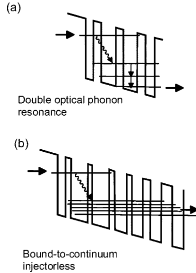
Fig. 5. New designs discussed in this article. The active regions are based on bound-to-continuum transition [30] or two phonon resonances [36].
