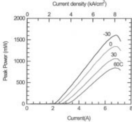
Fig. 9. Pulsed peak power versus injected current characteristics of a 3-mm long and 28- \mu\text{m} wide two-phonon resonance device. The device is driven at a low (1.5%) duty cycle.
