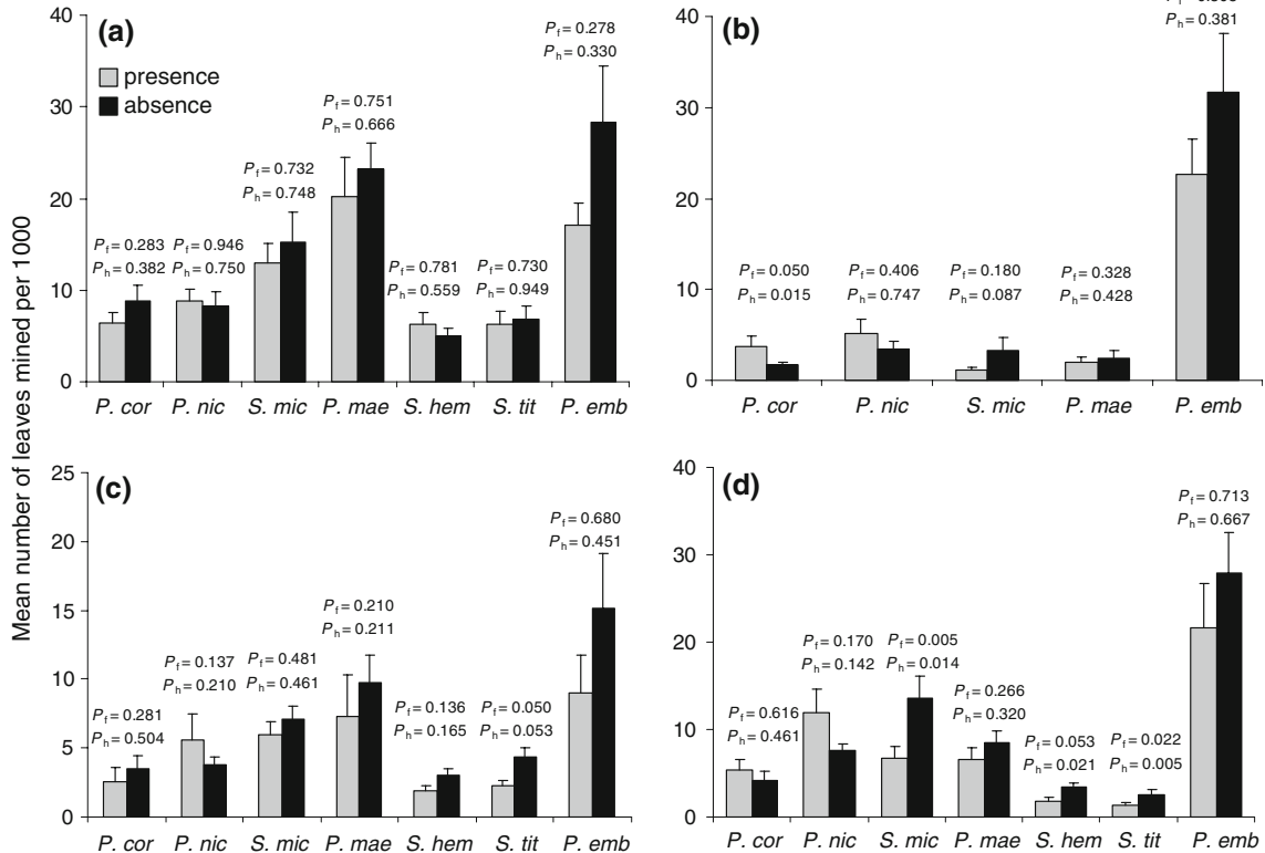
Fig. 3 Abundance of native leaf miners in Switzerland, in a July 2005, b September 2005, c July 2006 and d September 2006. Error bars represent standard errors. For the significance
