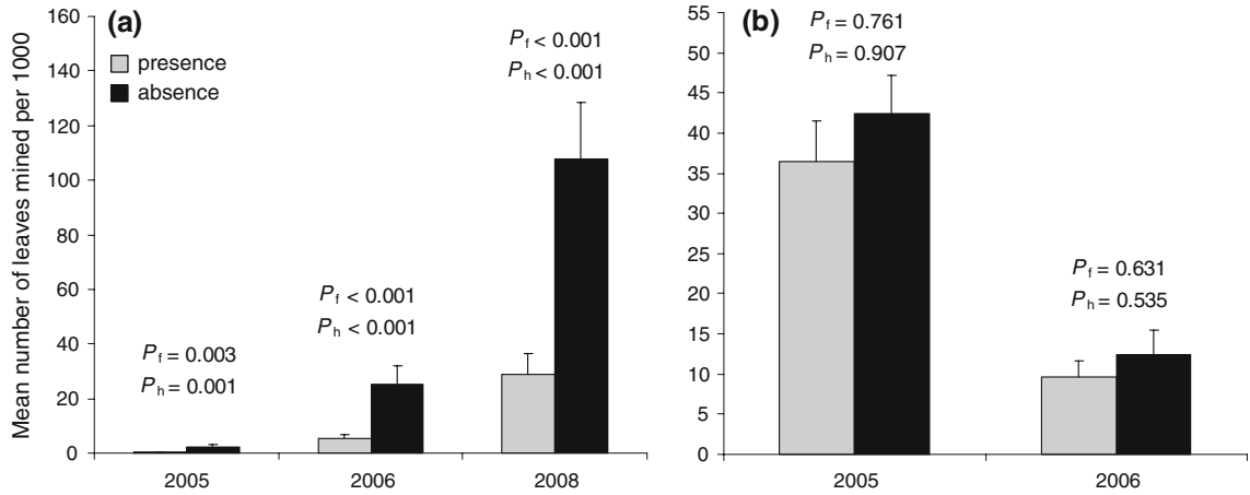
Fig. 2 Abundance of a Orchestes fagi (2005, 2006 and 2008) and b Aulagromyza hendeliana , (2005 and 2006) in presence and absence of Cameraria ohridella , in Switzerland. Error
