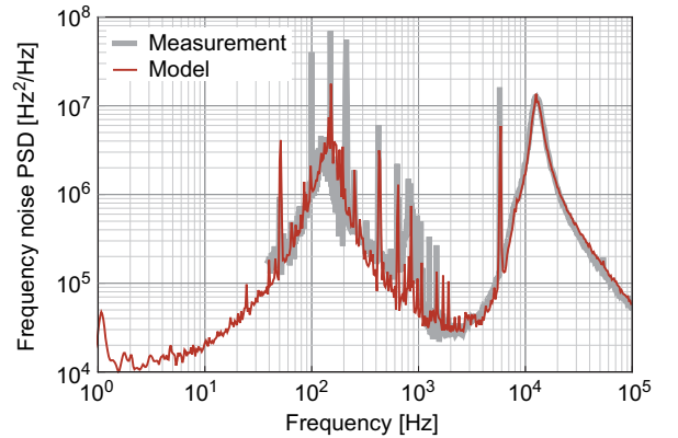
Fig. 7. (Color online) Comparison of the frequency noise of the CEO-free heterodyne beat ( \nu_N - f_{CEO} = N \cdot f_{rep} ) experimentally measured (thick grey curve) and calculated from the model (thin dark curve). In order to overcome the limitation in the frequency noise of the free-running repetition rate used in the model that results from the instrumental noise floor (see Fig. 5), the frequency noise PSD of f_{rep} was obtained from the CEO-free optical beat at 1.56 \mu\text{m} ( N \cdot f_{rep} with N \approx 770,000 ) divided by N^2 .
