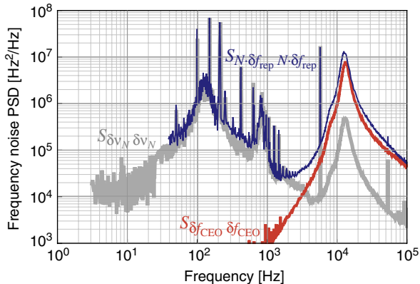
Fig. 6. (Color online) Measured individual contributions of the CEO and repetition rate frequency noise PSD ( S_{\delta f_{CEO} \delta f_{CEO}} and S_{N \cdot \delta f_{rep} N \cdot \delta f_{rep}} ) to an optical comb line at 1.56 \mu\text{m} and comparison with the measured frequency noise of the optical comb line ( S_{\delta v_N \delta v_N} ) experimentally assessed from the heterodyne beat with a cavity-stabilized laser.
