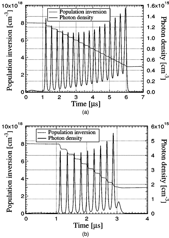
Fig. 7 Simulation of pulses with \beta_{\max}=11\text{ m}^{-1} and \beta_{\min}=3\text{ m}^{-1} where the rise times of the quality factor are (a) 5\text{ }\mu\text{s} and (b) 2\text{ }\mu\text{s} .
