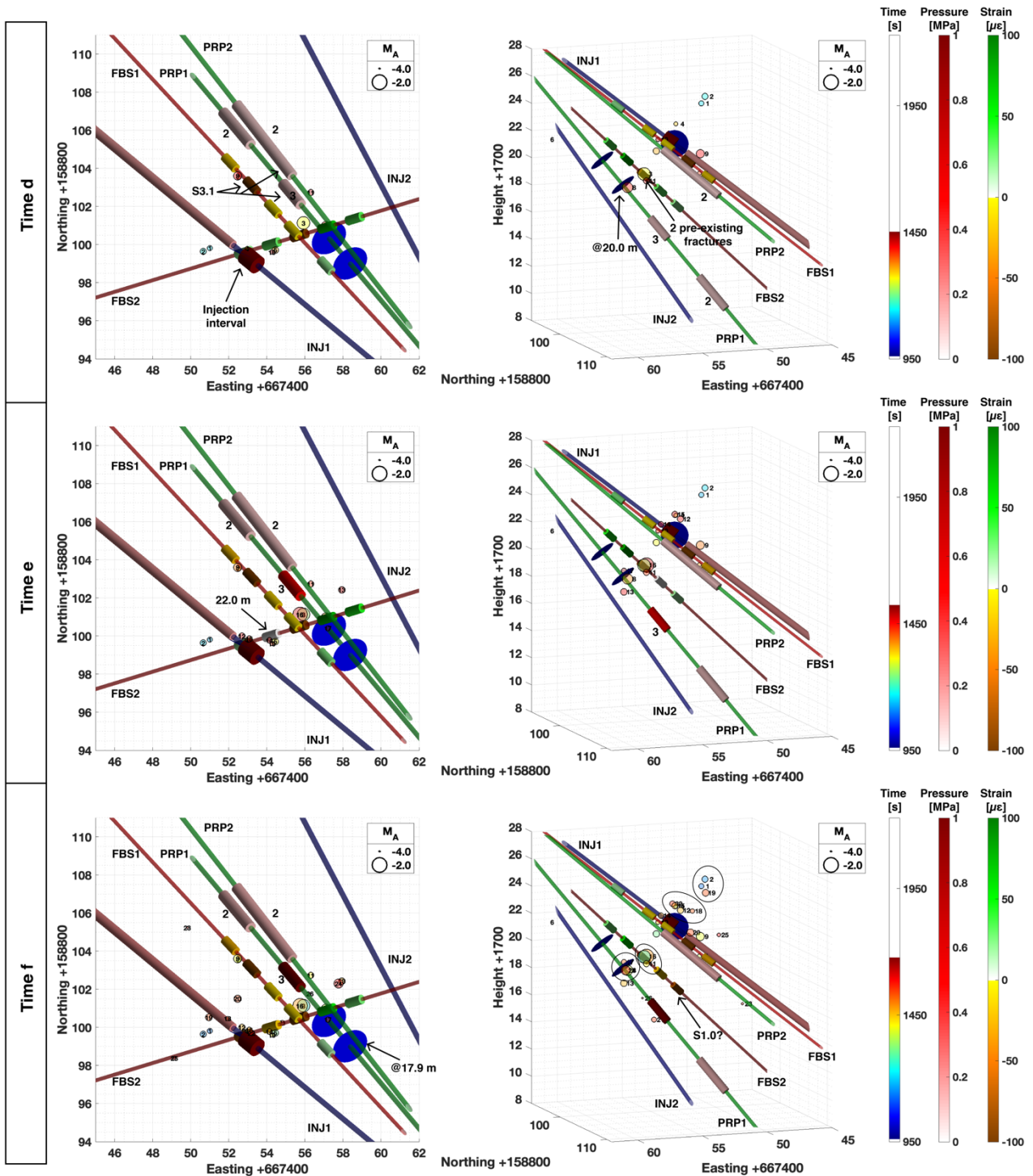
Figure 3: Seismo-hydrromechanical Observations Visualized Looking on Plane View (Left Column) and Parallel to the Shear Zones (Right Column). Each Row Represents a Temporal Resolved Snapshot at time d, e and f Presented in Figure 2d.
