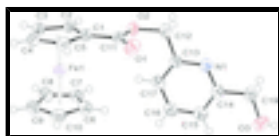
Fig. 1. The molecular structure of {6-(hydroxymethyl)pyridin-2-yl}methyl ferrocene-1-carboxylate. Displacement ellipsoids are drawn at the 50% probability level.
