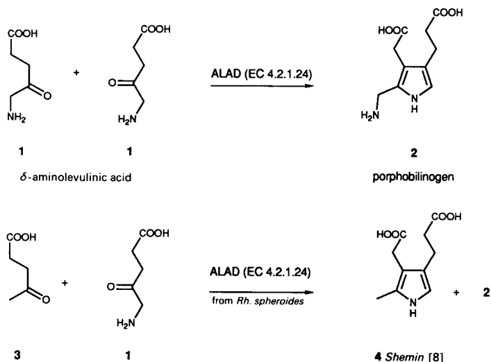
Scheme 1. Enzymatic Formation of Porphobilinogen 2 and Pyrrole 4 [4] [5] [8]
