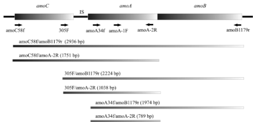
Fig. 1. Structure of the amoCAB operon and position of the primers used in this study. Initial PCR amplification with six different primer pairs was used to generate templates for nested amoA amplification. The predicted size of the PCR products is in parentheses.
