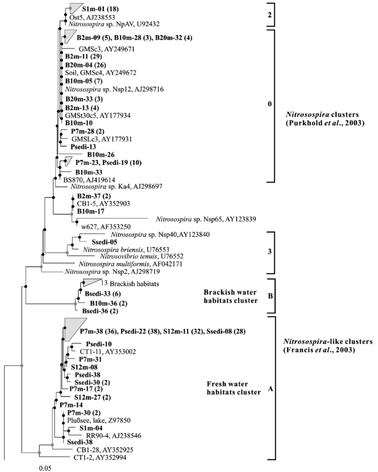
Fig. 3. Fitch–Margoliash phylogenetic tree calculated in ARB with 248 amino acids of AmoA using PmoA from Crenothrix polyspora (Acc. no. DQ295904) as an outgroup. Nomenclature of clusters according to Purkhold et al. (2003) and Francis et al. (2003). Clones from this study are in bold, with the number of identical clones in parentheses and their origin coded with three different letters: B for Baltic Sea, P for Plußsee and S for Schöhsee. Bootstrap values for \geq 90 replicate trees are indicated at the nodes with three different colors: black (100%), gray (95–99%) and white (90–94%).
