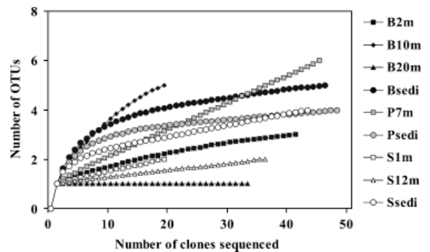
Fig. 2. Rarefaction curves of amoA -based OTUs at 5% cutoff at the DNA level. Coding of the samples with three different colors: black, Baltic Sea; gray, Plußsee; white, Schöhsee.
