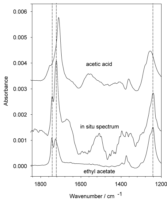
Fig. 7. ATR spectra of acetic acid and ethyl acetate dissolved in ethanol. The spectra were recorded over a clean ZnSe internal reflection element. The reference was recorded in neat ethanol. For comparison an in situ ATR spectrum of a Pd/Al 2 O 3 catalyst in contact with ethanol is shown. The spectrum was recorded five seconds after switching to O 2 -saturated ethanol (see Fig. 2 for more details).
