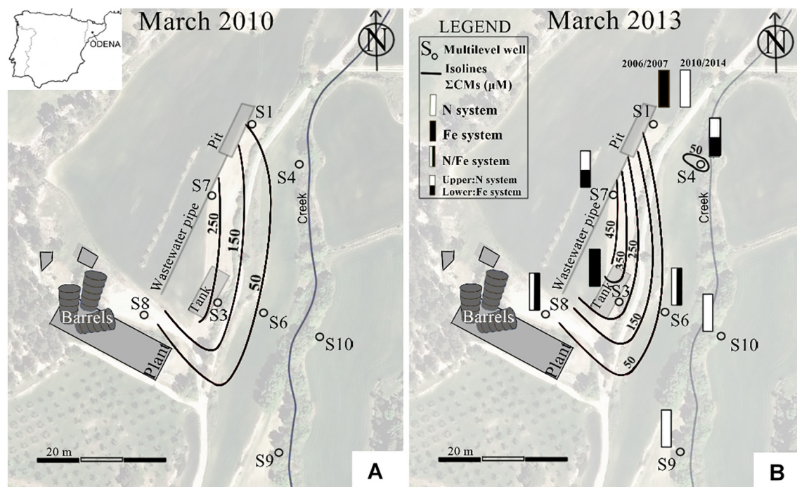
Fig. 1. Ôdena site map and groundwater monitoring wells network (S1–10). Groundwater flow system from Palau et al. (2014) was used to draw a simplified contamination CMs plume evolution (sum of molar concentrations of CT, CF and DCM at the most contaminated level for each well) from A) March 2010 to B) March 2013. The barrels from chemical plant, the tank, pit and the wastewater pipe were all removed in 2005 but are shown in the map for a better understanding. Rectangles in B represent the well's Eh-controlling system from 2006 to 2014, determined after analysing the Eh-pH diagrams (Fig. A1), calculated with data from field samples over time (Table A1). N system means equilibrium between nitrogen (N) chemical species of the N-H 2 O system and Fe system, equilibrium between iron (Fe) chemical species of the Fe-S-C-H 2 O system, according to Eh and pH values measured in each well. If changes in the redox conditions of a well were detected in Eh-pH diagrams (Fig. A1) in depth (i.e. S4 and S7) or over time (i.e. S1) they are also specified in the figure.
