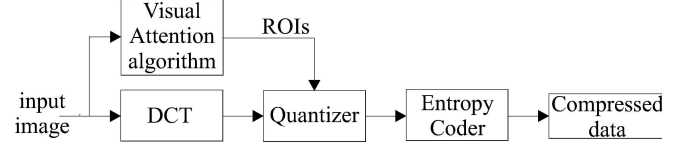
Figure 3. Adaptive JPEG-based Image compression Algorithm
