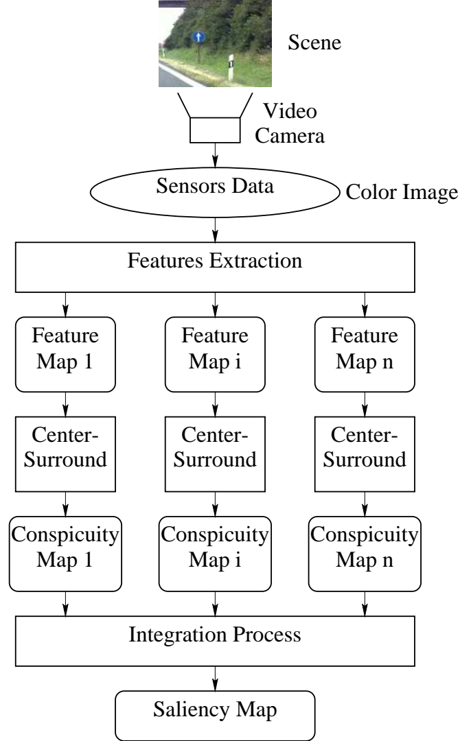
Figure 1. Scheme of a computational model of attention.
