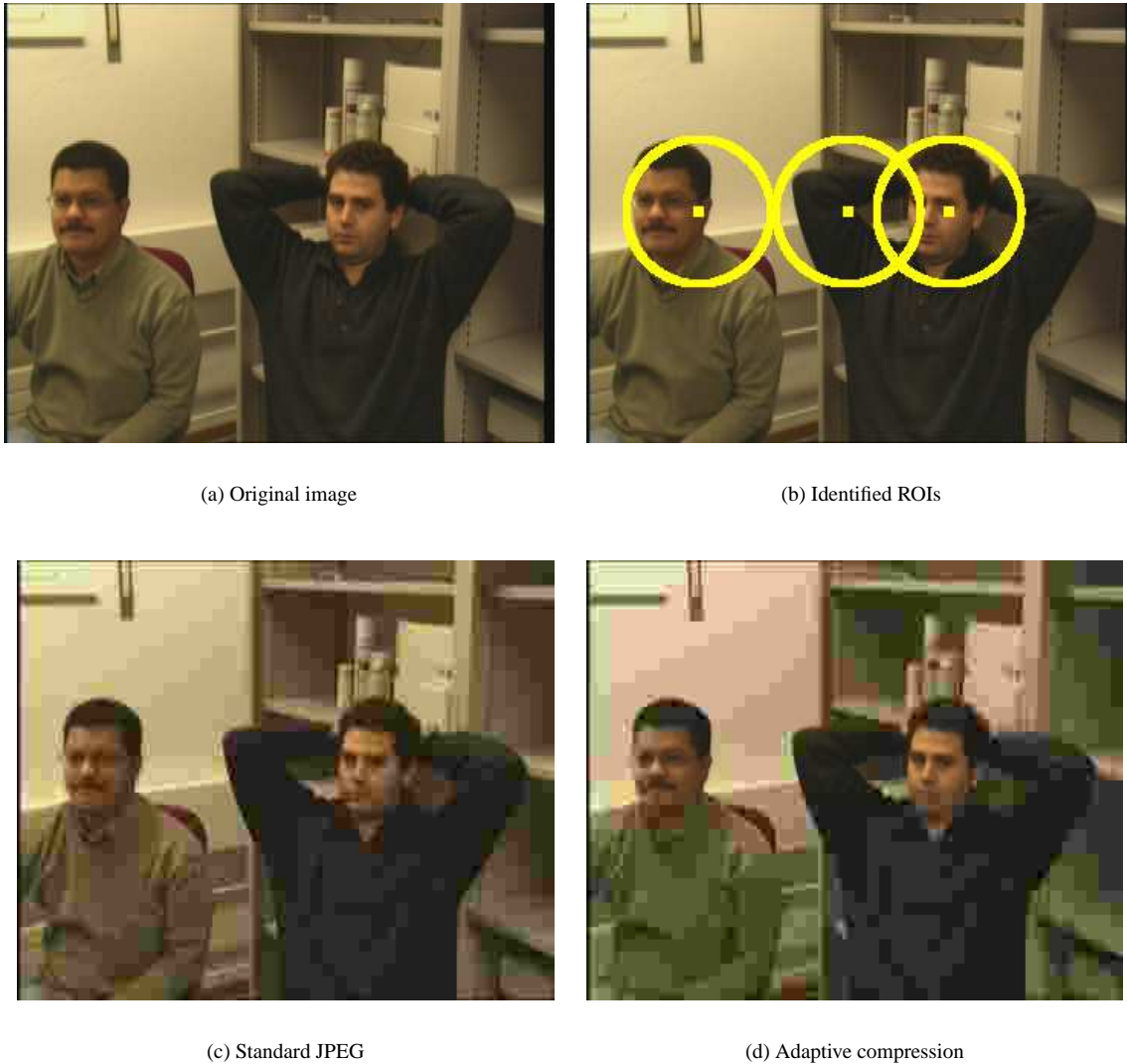
Figure 6. Adaptive versus non-adaptive compression: Example 2.
