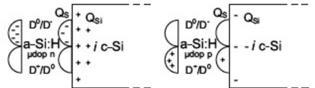
FIG. 11. Sketch of the average state of charge of the recombination centers in microdoped a-Si:H layers passivating intrinsic c-Si: n -type \mu\text{dop} is shown on the left, p -type \mu\text{dop} on the right (charge density is adapted to measurements). The sketched occupation level in the a-Si:H distant from the interface in the drawings illustrates the expected “bulk” occupation in microdoped a-Si:H layers.
