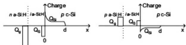
FIG. 12. Sketch of the charge distribution when passivating lightly p -type doped c-Si by stacks of i/n a-Si:H (left hand) or i/p a-Si:H (right hand).
