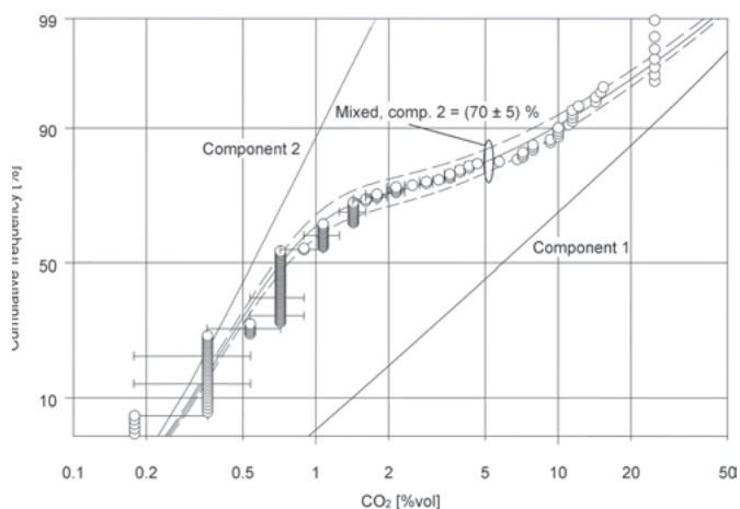
Fig. 7. \text{CO}_2 in soil gas frequency distribution and approximation by a 2-component model. Component 2: \text{CO}_2 production in the soil; component 1: geogenetic production. Maximum measured values are limited to 25 vol.%, the full scale of the instrument used. Error bars are 1- \sigma uncertainty estimations.
