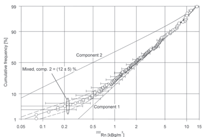
Fig. 8. ^{222}\text{Rn} in soil gas frequency distribution and approximation by a 2-component model. Component 1: typical radon production in an average Swiss soil. There is no need for any radon from deep down to explain the distribution. Component 2 with a lower median and a broader distribution may be due to leaky sampling. Error bars are 1-sigma counting statistics.
