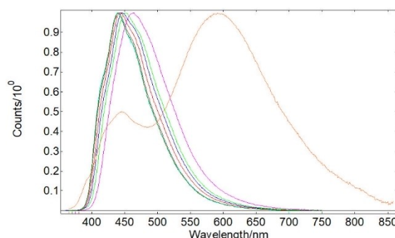
Figure 2. Normalized emission spectra of R IPP-BF 2 compounds recorded in solution (CH 2 Cl 2 , 5 · 10 −5 M). (■), H IPP-BF 2 ; (■), Me IPP-BF 2 ; (■), MeO IPP-BF 2 ; (■), F IPP-BF 2 ; (■), Cl IPP-BF 2 ; (■), Br IPP-BF 2 ; (■), I IPP-BF 2 ; (■), NO2 IPP-BF 2 . (checked, it's ok)
