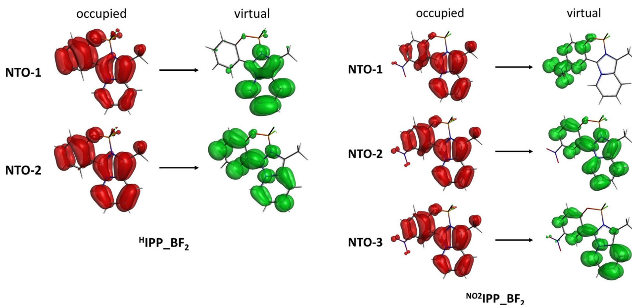
Figure 4. Natural Transition Orbitals (NTOs) calculated for compounds {}^1\text{IPP\_BF}_2 and {}^{\text{NO}_2}\text{IPP\_BF}_2 relative to the first (NTO-1), second (NTO-2) and (for {}^{\text{NO}_2}\text{IPP\_BF}_2 ) third (NTO-3) low energy transitions (see text).
