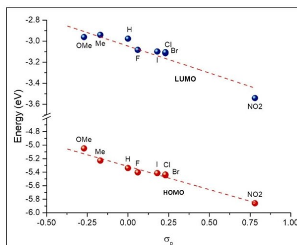
Figure 6. HOMO (red) and LUMO (blue) energies of R IPP-BF 2 vs. Hammett's σ p of substituent R. Linear fit: R 2 = 0.916 and 0.967 respectively for LUMO and HOMO.
