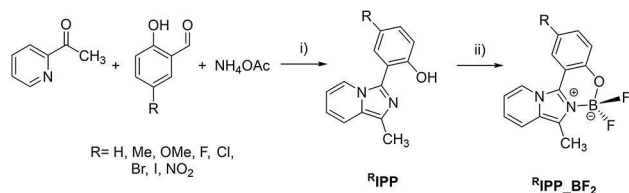
Scheme 1. Synthesis of R IPP and reaction with boron trifluoride diethyletherate to obtain R IPP·BF 2 . i) 2-Acetylpyridine:aldehyde:NH 4 OAc 1:2:5; AcOH, r.t., 7 days. ii) BF 3 ·Et 2 O, Et 3 N, CH 2 Cl 2 , r.t.
