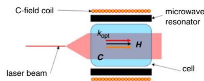
Fig. 1 Schematic representation of fields' orientations required for CW-DR atomic clock. \mathbf{k} , light propagation vector; \mathbf{H} , microwave magnetic field; \mathbf{C} , static magnetic field
