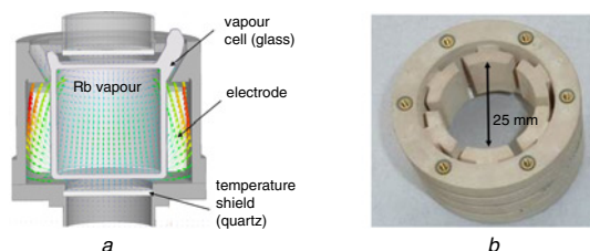
Fig. 2 Details of cavity
