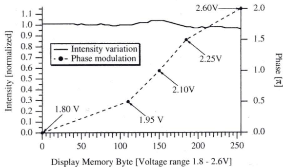
Fig. 1. Measured phase shift and intensity variation versus addressing voltage of the LCTV. The addressing voltage does not vary linearly with the display memory byte.
