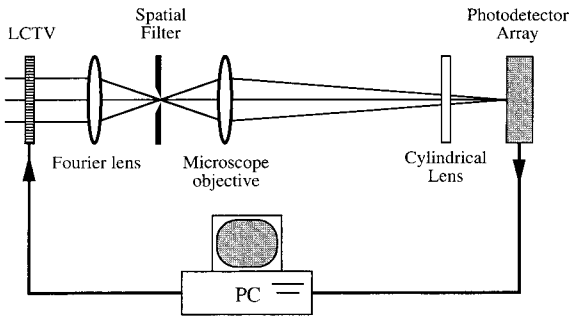
Fig. 3. Schematic of the optical parallel processor. The Fourier lens, f=380 mm, transforms the information displayed on the LCTV. The microscope objective images the Fourier plane onto the photodetector array with about 50\times magnification. The cylindrical lens adapts the rectangular diffraction pattern, due to the asymmetric spacing of the LCTV pixels ( 80\ \mu\text{m}\times 90\ \mu\text{m} ), to the square format of the photodetector array.
