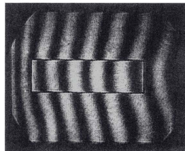
Fig. 2. LCTV in a Mach-Zehnder interferometer displaying \pi phase modulation.
