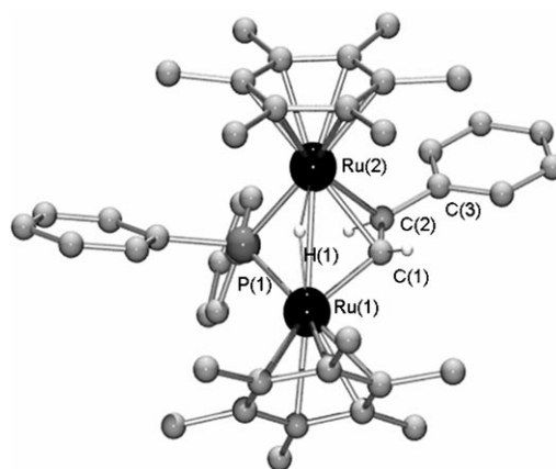
Figure 5. Molecular structure of [(C 6 Me 6 ) 2 Ru 2 (PPh 2 )(CHCHPh)H] + ( 2 ); the hydrogen atoms and tetrafluoroborate molecule are omitted for clarity. Selected bond lengths (Å) and angles (°): Ru(1)-Ru(2) 2.7923(6), Ru(1)-P(1) 2.2900(9), Ru(2)-P(1) 2.3171(11), Ru(1)-C(1) 2.032(4), Ru(2)-C(1) 2.180(4), Ru(2)-C(2) 2.387(4), C(1)-C(2) 1.374(6); Ru(1)-P(1)-Ru(2) 74.61(3), Ru(1)-C(1)-Ru(2) 82.97(16), Ru(1)-C(1)-C(2) 128.7(3), C(1)-C(2)-C(3) 126.1(3).
