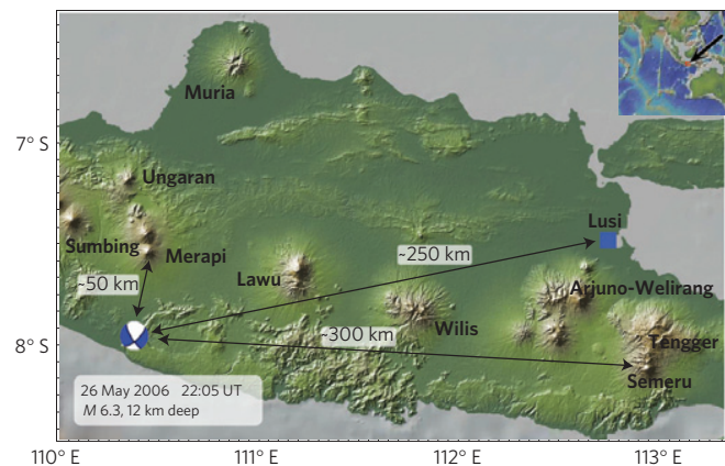
Figure 1 | Map of Java with relevant distances from the Yogyakarta earthquake. The blue square marks the position of Lusi and arrows show the distance between the epicentre of the Yogyakarta earthquake and the systems that responded to that event.
