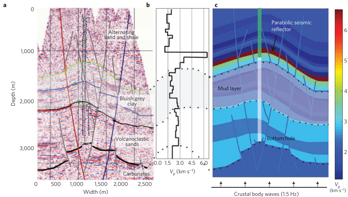
Figure 2 | Geometry, V_p variations with depth and model of Lusi used in the numerical study. a , Seismic profile of the geological structures 8 beneath Lusi used to reconstruct the geology of the model. b , Vertical profile for V_p velocities used in the model 10 . The acoustic impedance of faults is not known, so we assumed \rho = 2,000 \text{ kg m}^{-3} , V_p = 2,325 \text{ m s}^{-1} and V_s = 1,531 \text{ m s}^{-1} . c , Distribution of V_p velocities in the model domain. The mud layer is shaded grey, the cased and uncased well (not modelled) are shaded green and white, respectively.
