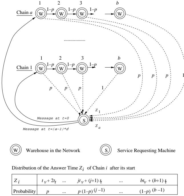
Figure 4: Message Transmission and their Probabilities in the used Model
