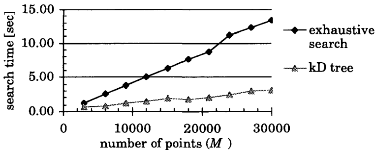
Figure 3.7 Search time using a kD tree
