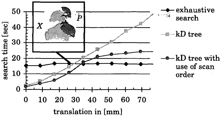
Figure 3.8 Limits of kD tree search routine
