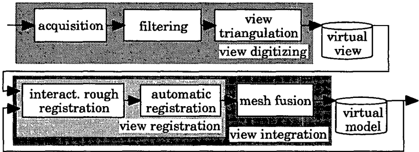
Figure 5.1 Digitizing system architecture
