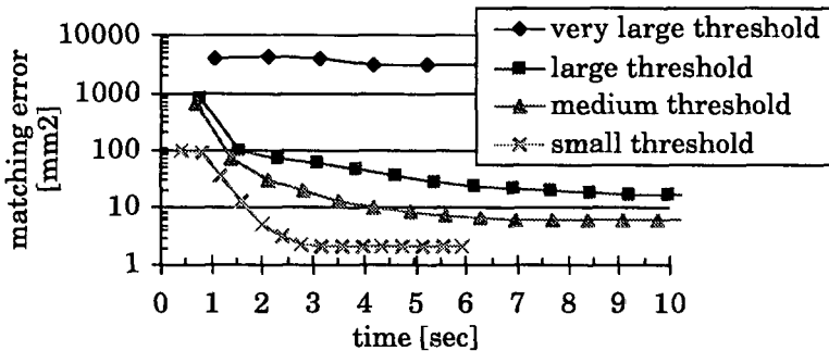
Figure 5.11 Matching convergence for different geometric thresholds
