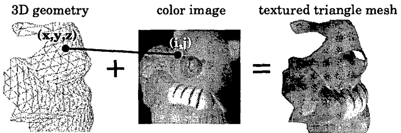
Figure 2.10 Color texture image mapping
