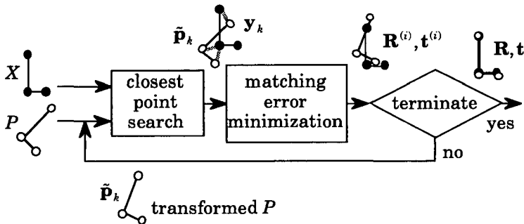
Figure 3.1 Data flow of ICP algorithm
