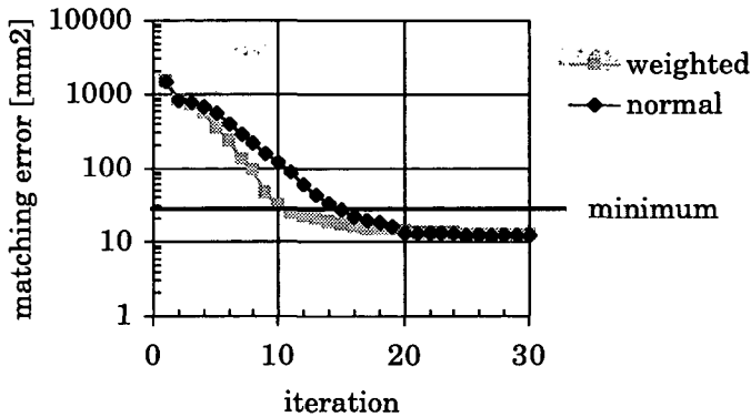
Figure 4.15 Matching acceleration with weighted couplings
