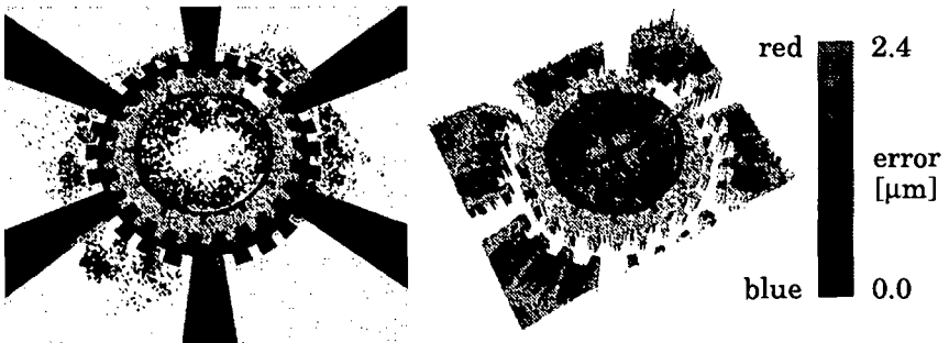
Figure 6.4 Augmented reality showing the matching errors for a micromotor
