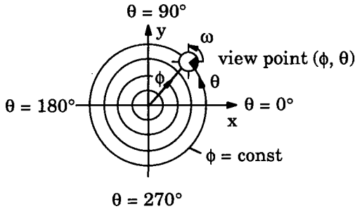
Figure 3.15 Definition of the SIC-map
