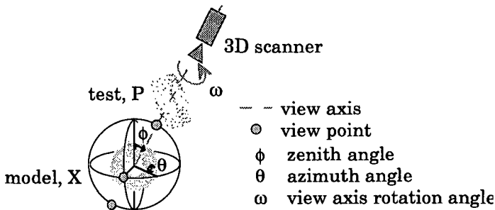
Figure 4.3 Recognition setup for the geometric point matching
