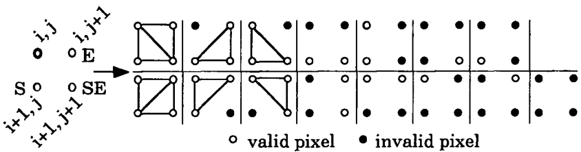
Figure 2.8 Range image triangulation
