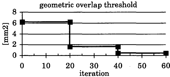
Figure 5.6 Typical values of overlap threshold over several ICP iterations
