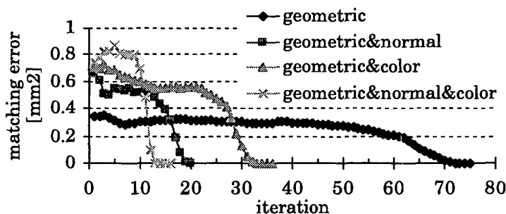
Figure 5.9 Convergence of ICP using multiple features
