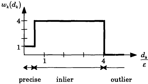
Figure 4.14 Weight function for closest point couplings
