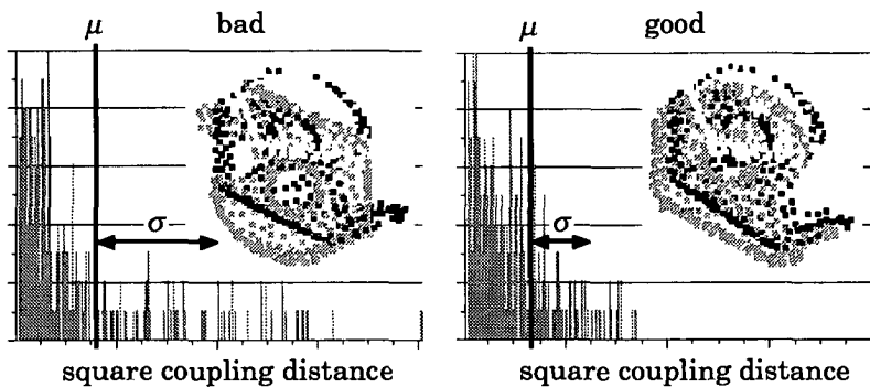
Figure 4.12 Distance histogram of closest points for two matching cases
