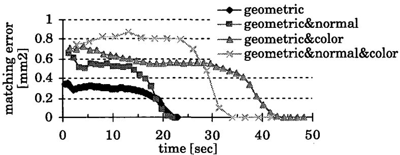
Figure 5.10 Absolute execution time of ICP using multiple features
