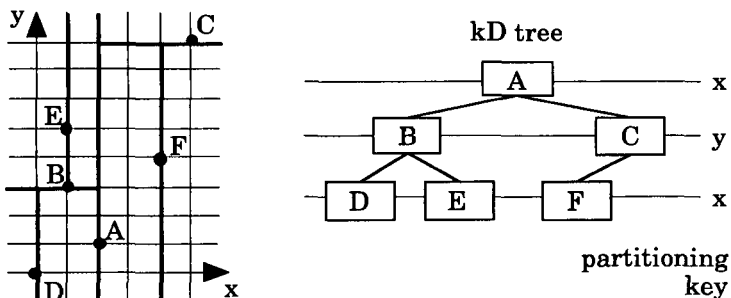
Figure 3.6 Example of a 2D tree construction
