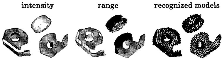
Figure 4.4 Recognition results for scotch dispenser parts
