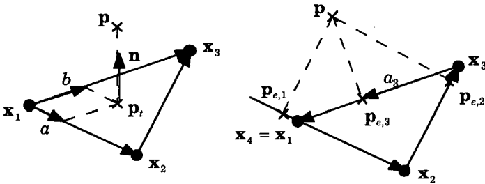
Figure 3.10 Closest point to triangle distances
