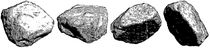
Figure 5.19 Antique brick
