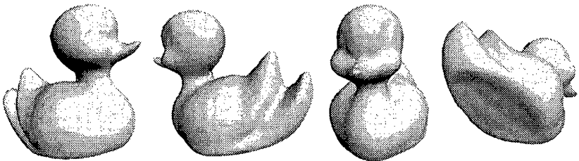
Figure 5.18 Toy duck
