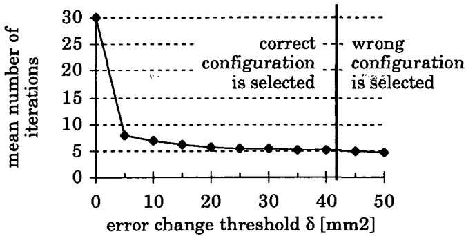
Figure 4.13 Fast initial configuration selection with error change
