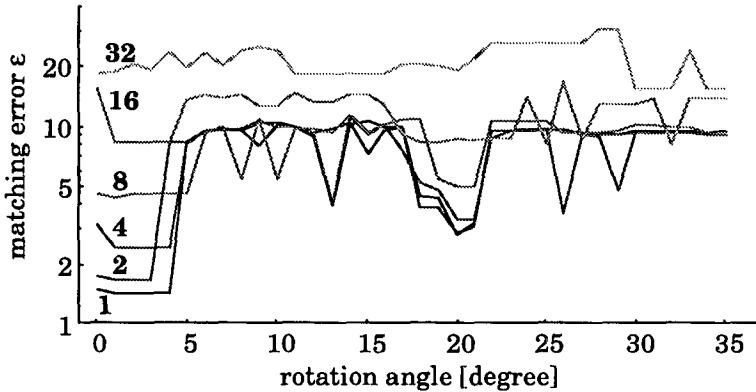
Figure 4.17 Matching errors for different reduction factors
