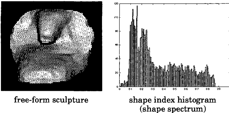
Figure 2.2 Appearance-based representation of a sculpture [DOR]
