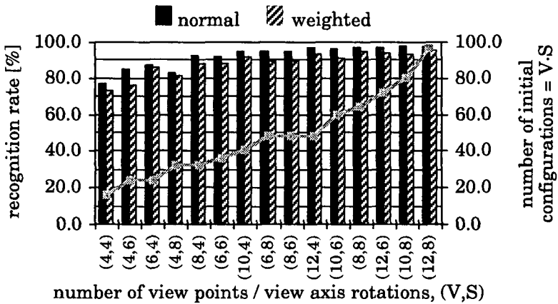
Figure 4.19 Recognition performance and cost for different setups
