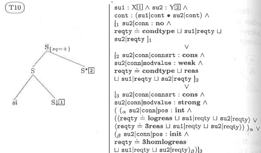
FIGURE 10 Conditional sentences 18
