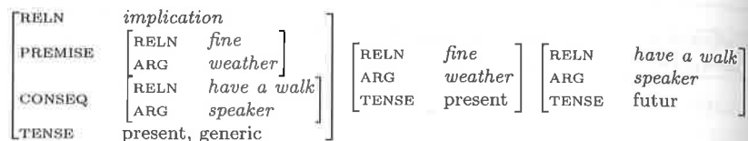
FIGURE 4 Information structure
