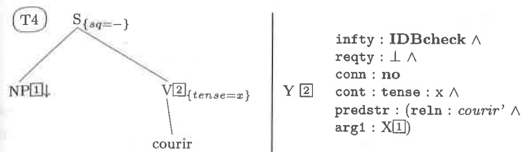
FIGURE 5 Simple sentences
