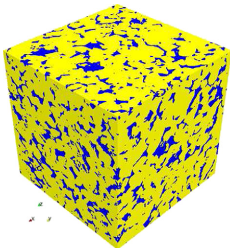
Fig. 8. The micro CT of a sample of Berea sandstone used as a 3D reference. In the image, of size 400 \times 400 \times 400 voxels, the blue represents the pores and the yellow the matrix. (For interpretation of the references to color in this figure legend, the reader is referred to the web version of this article.)
