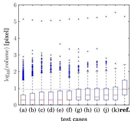
Fig. 15. The \log_{10} of the volume of the pores computed on the simulations of the micro CT image shown in Fig. 12a–12k. The simulations are obtained with the paBor method and with a different value of the weights w_{1,2} for each test case. The weights vary from 0.1 (a) to 2.0 (k). The dashed line represents the median of the volume of the geobodies contained in the reference image.
