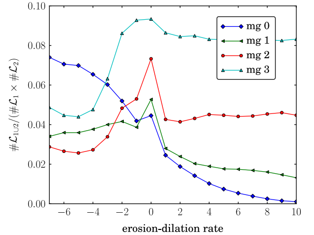
Fig. 23. The ratio between the size of the merged list \mathcal{L}_{1,2} and the size of the merged list under the hypothesis that all the elements of the two merged lists \mathcal{L}_1 and \mathcal{L}_2 are compatible. The list \mathcal{L}_1 is computed from the training image of Fig. 22h, while the list \mathcal{L}_2 is obtained from the same image eroded or dilated (Fig. 22). The sizes of the merged lists are computed for four different multigrid levels.
