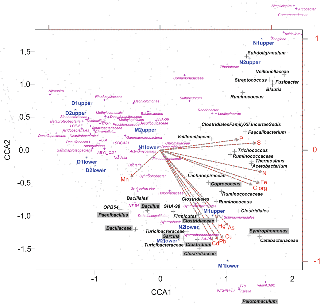
Fig. 4 Canonical correspondence analysis (CCA) triplot of the samples ( blue text and dots ) based on the bacterial groups identified in the sediment of the Vidy Bay and constrained by environmental variables. The ordination plot of the samples was constructed with results of OTUs picking and identification with the program QIIME from pyrosequencing data. Each OTU is represented by a cross in the plot. OTUs from sequences corresponding to less than 1 % (non
