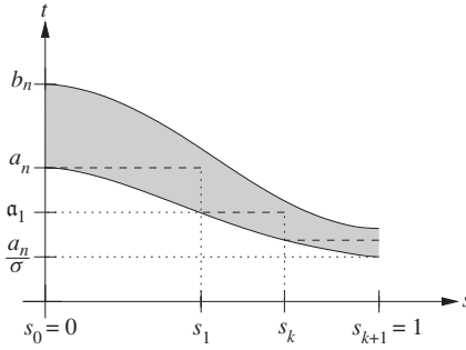
Fig. 3. The curves a_n(s) and b_n(s) .
